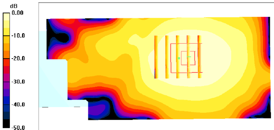
0 dB = 0.055mW/g
