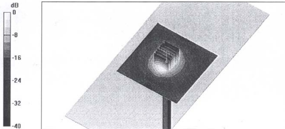
0 dB = 15.2 mW/g
