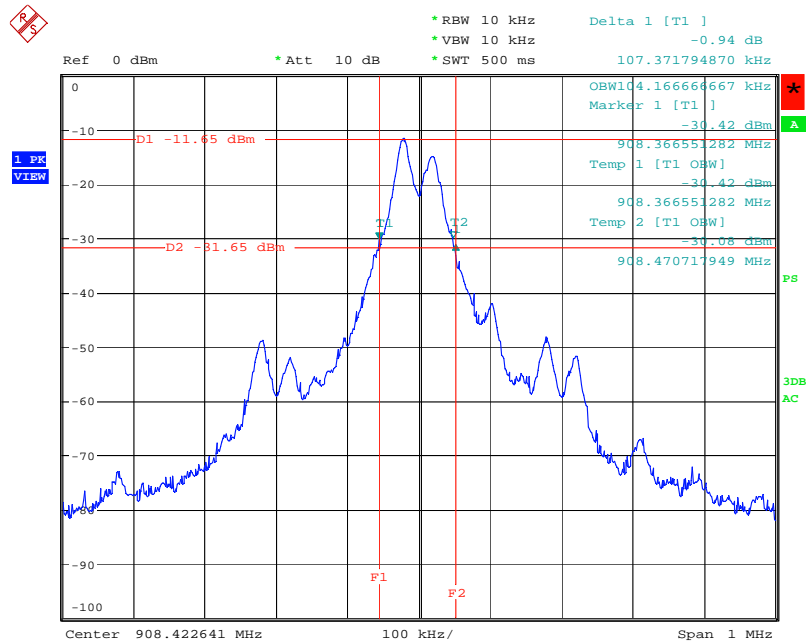
20 dB/99% Bandwidth Plot on 908.4 MHz
