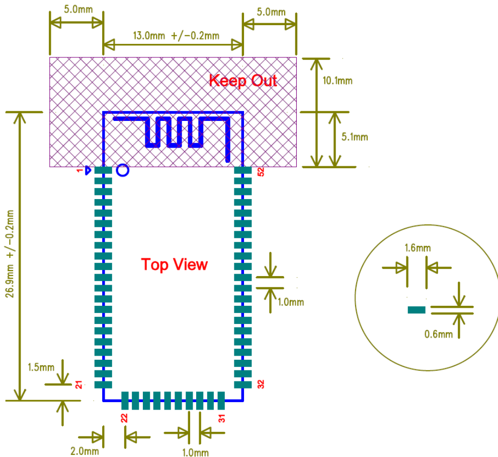
Figure 34: FSC-BT806Bfootprint
