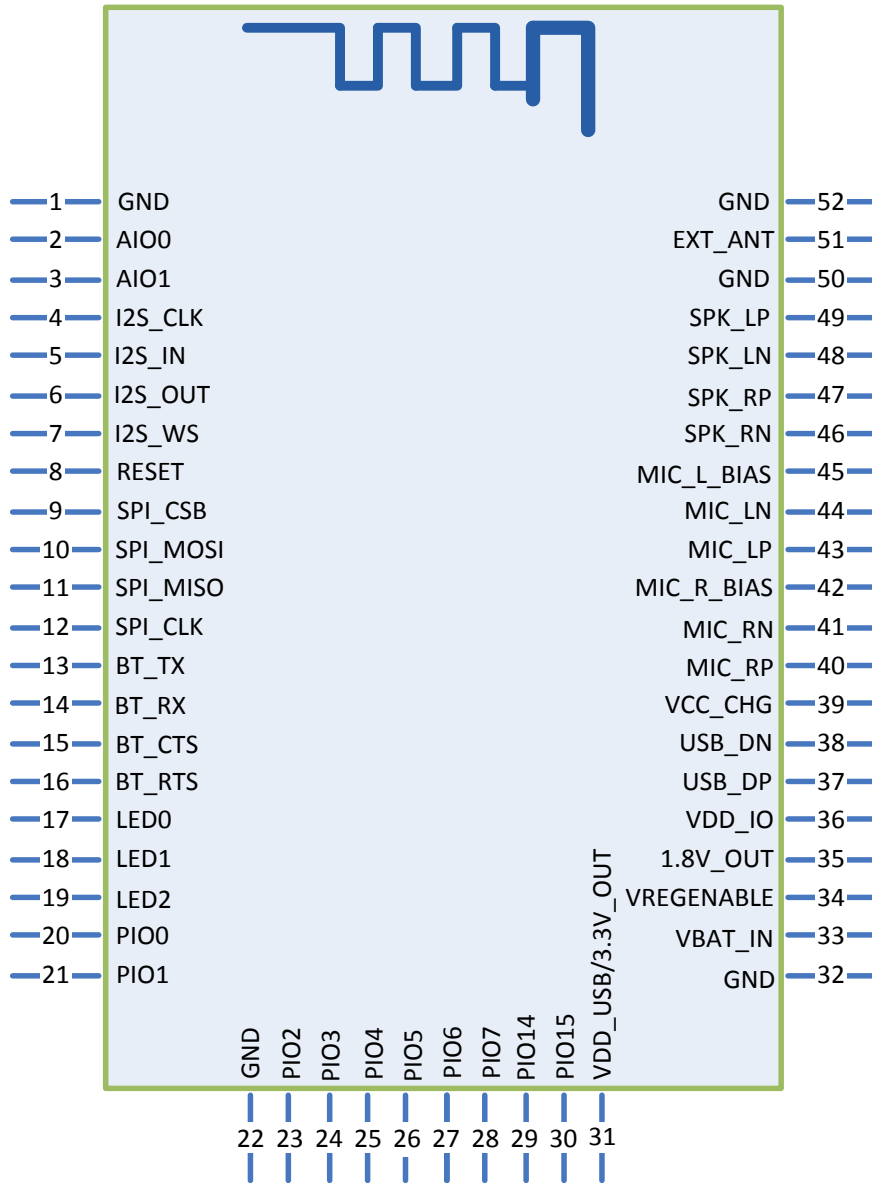
Figure 3: FSC-BT806BB PIN Diagram(Top View)
