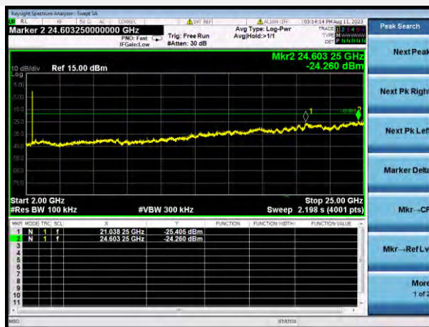
GFSK (BLE 1Mbps) MIDDLE CHANNEL, SPURIOUS 2 GHz ~ 25 GHz
