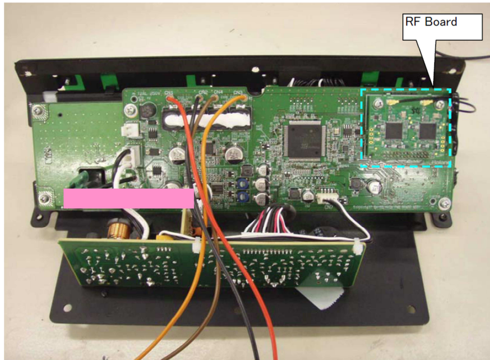
PWB Position
