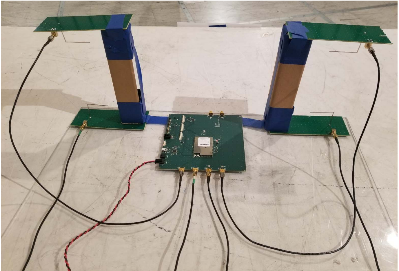
Figure 1.1-5:Module with Antennas)
