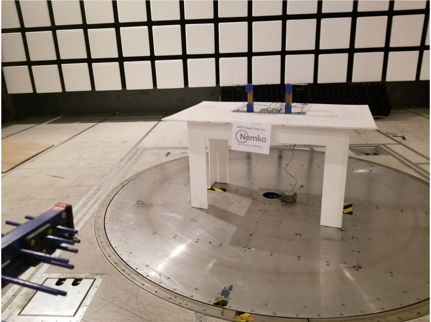
Figure 1.1-2: Radiated Emissions setup photo Front (30MHz-1GHZ)
