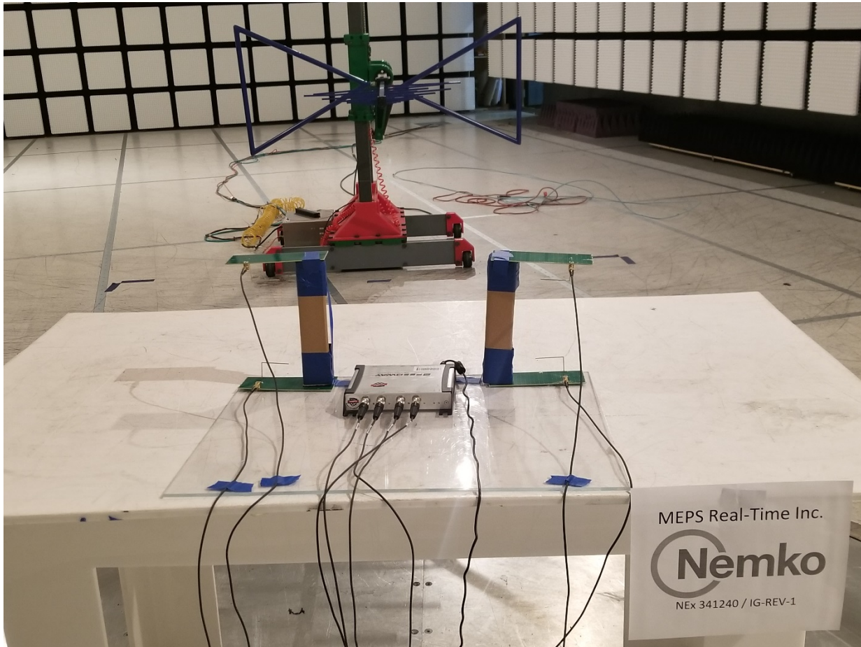
Figure 1.1-1: Radiated Emissions setup photo Back (30MHz-1GHZ)
