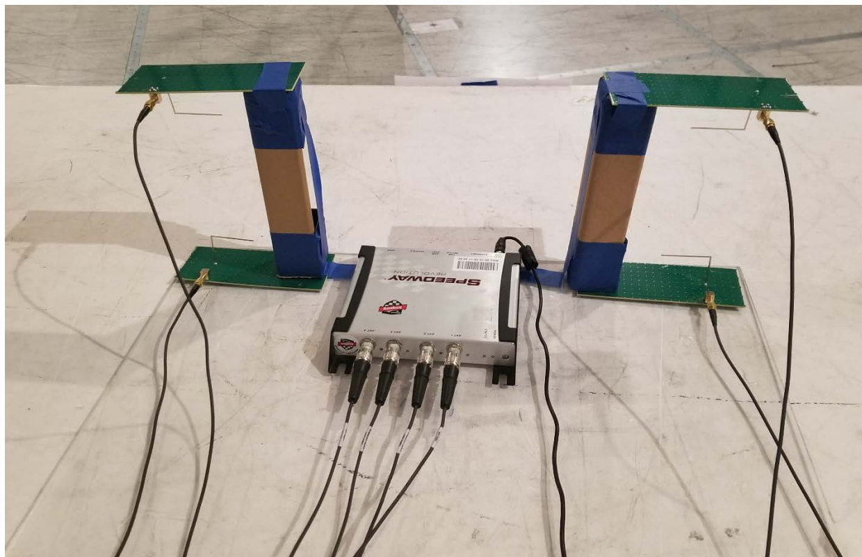
Figure 1.1-5:Module with Antennas
