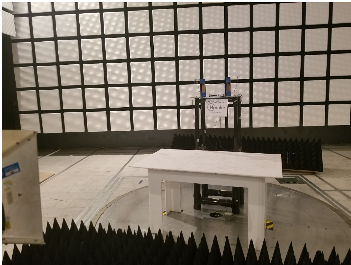
Figure 1.1-4: Radiated Emissions setup photo Front (1GHz-18GHZ)
