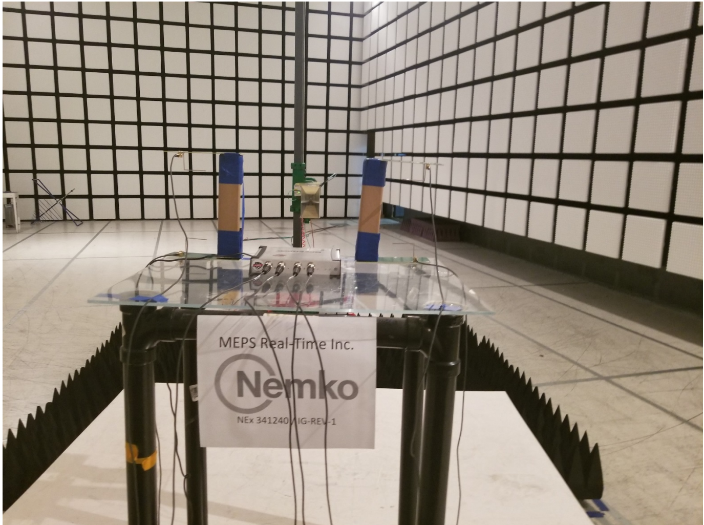
Figure 1.1-3: Radiated Emissions setup photo Back (1GHz-18GHZ)
