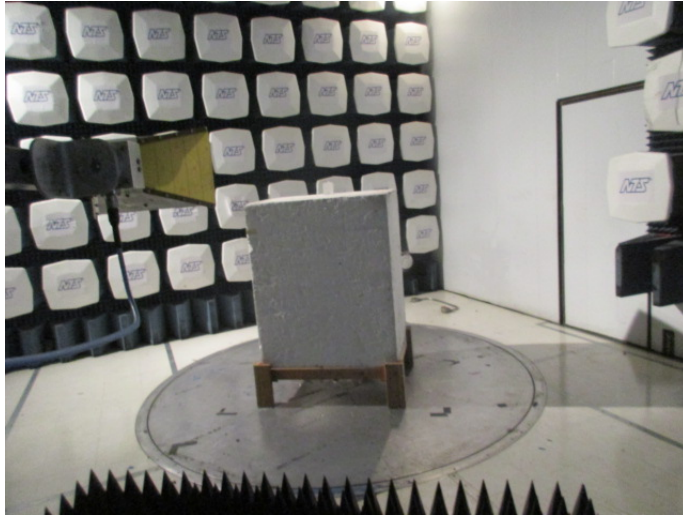
Radiated Spurious Emissions > 1GHz
