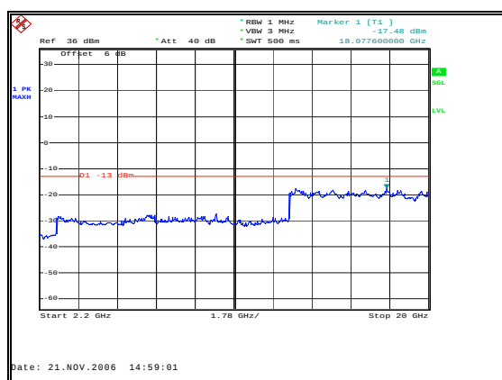
Figure 42: Spurious Emissions - Uplink GSM Low Channel – 2.2 GHz to 20 GHz
