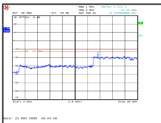
Figure 37: Spurious Emissions - Uplink CW Low Channel – Inter-modulation - 2 GHz to 20 GHz
