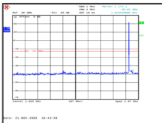
Figure 36: Spurious Emissions - Uplink CW Low Channel – Inter-modulation - 30 MHz to 2 GHz
