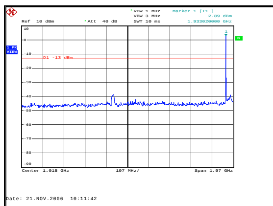
Figure 64: Spurious Emissions - Downlink CW Low Channel – Inter-modulation-30 MHz to 2 GHz
