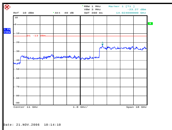
Figure 68: Spurious Emissions - Downlink CW High Channel–Inter-modulation-2 GHz to 20 GHz
