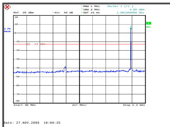
Figure 58: Spurious Emissions - Downlink TDMA Mid Channel – 30 MHz to 2.2 GHz
