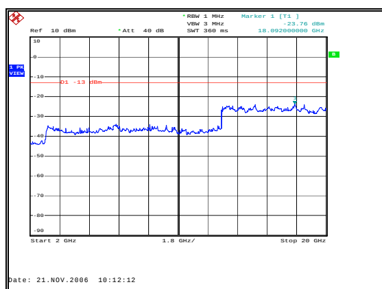
Figure 65: Spurious Emissions - Downlink CW Low Channel – Inter-modulation-2 GHz to 20 GHz
