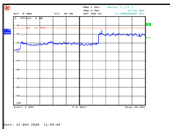
Figure 29: Spurious Emissions - Uplink TDMA Low Channel – Inter-modulation-2 GHz to 20 GHz
