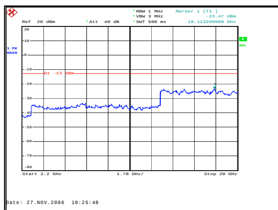
Figure 70: Spurious Emissions - Downlink GSM Low Channel – 2.2 GHz to 20 GHz
