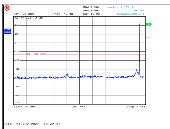
Figure 39: Spurious Emissions - Uplink CW High Channel – Inter-modulation - 30 MHz to 2 GHz
