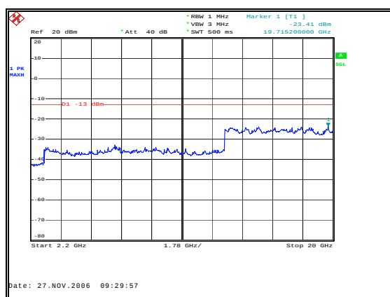
Figure 51: Spurious Emissions - Downlink CDMA Mid Channel – 2.2 GHz to 20 GHz
