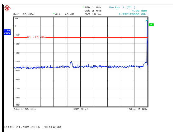
Figure 67: Spurious Emissions - Downlink CW High Channel–Inter-modulation-30 MHz to 2 GHz
