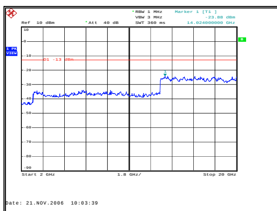
Figure 54: Spurious Emissions-Downlink CDMA High Channel-Inter-modulation-2GHz to 20GHz
