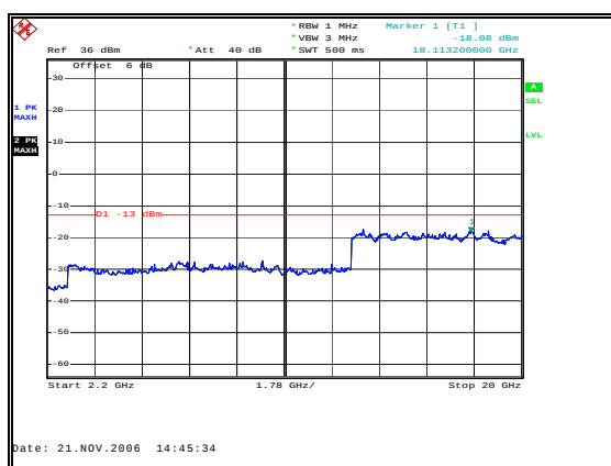
Figure 31: Spurious Emissions - Uplink TDMA Mid Channel – 2.2 GHz to 20 GHz
