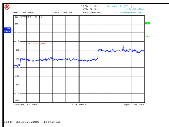
Figure 40: Spurious Emissions - Uplink CW High Channel – Inter-modulation - 2 GHz to 20 GHz
