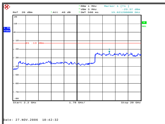
Figure 72: Spurious Emissions - Downlink GSM Mid Channel – 2.2 GHz to 20 GHz
