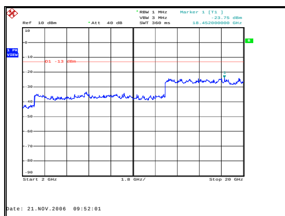
Figure 57: Spurious Emissions-Downlink TDMA Low Channel–Inter-modulation-2GHz to20 GHz
