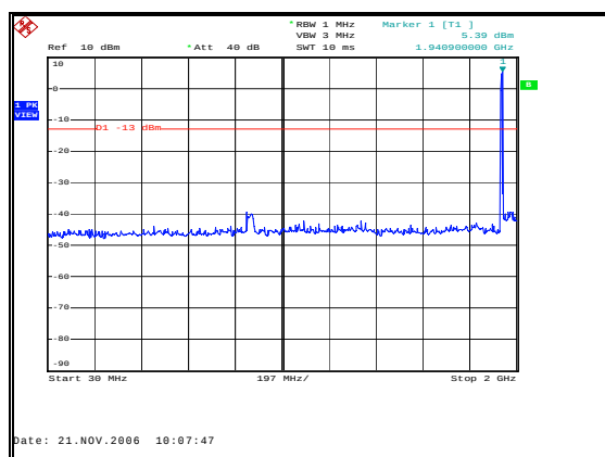
Figure 48: Spurious Emissions-Downlink CDMA Low Channel–Inter-modulation-30MHz to 2GHz
