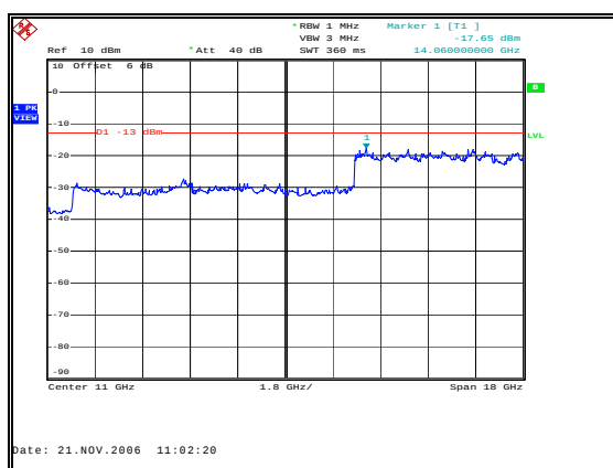
Figure 34: Spurious Emissions - Uplink TDMA High Channel – Inter-modulation-2 GHz to 20 GHz
