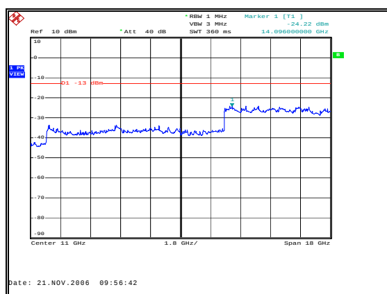
Figure 62: Spurious Emissions-Downlink TDMA High Channel-Inter-modulation-2GHz to 20GHz
