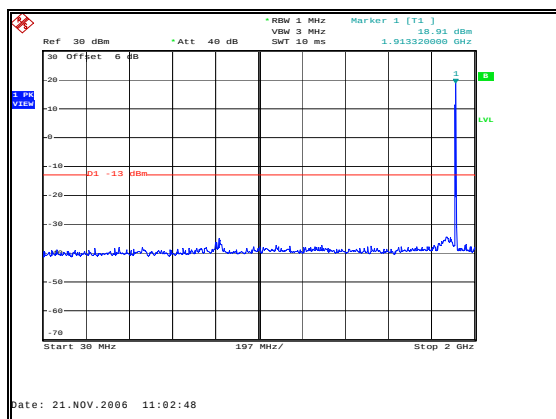
Figure 33: Spurious Emissions - Uplink TDMA High Channel – Inter-modulation-30 MHz to 2 GHz
