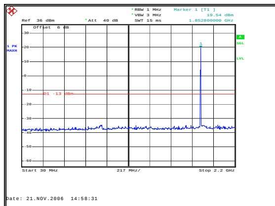
Figure 41: Spurious Emissions - Uplink GSM Low Channel – 30 MHz to 2.2 GHz
