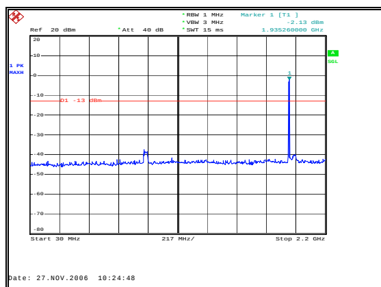
Figure 69: Spurious Emissions - Downlink GSM Low Channel – 30 MHz to 2.2 GHz
