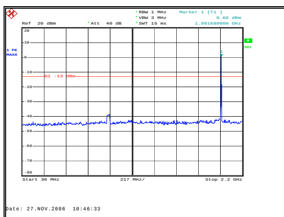
Figure 73: Spurious Emissions - Downlink GSM High Channel – 30 MHz to 2.2 GHz
