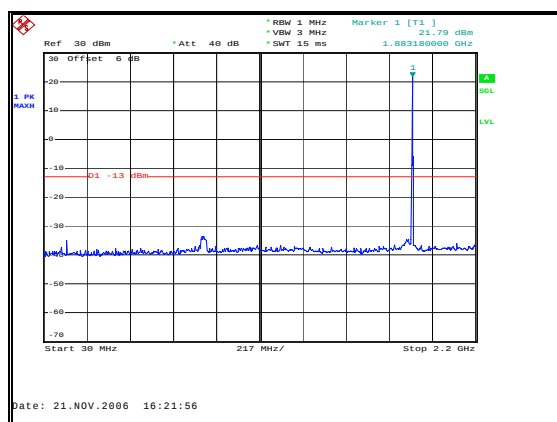
Figure 43: Spurious Emissions - Uplink GSM Mid Channel – 30 MHz to 2.2 GHz
