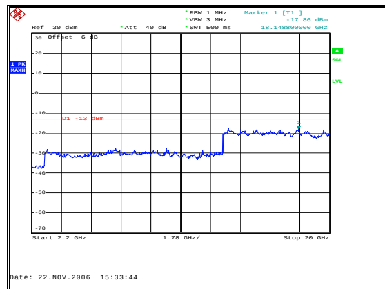
Figure 46: Spurious Emissions - Uplink GSM High Channel – 2.2 GHz to 20 GHz
