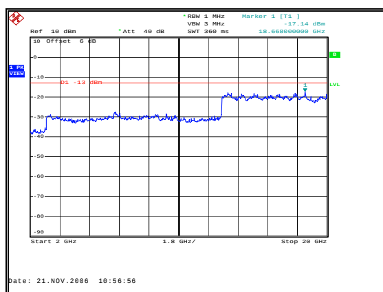
Figure 26: Spurious Emissions - Uplink CDMA High Channel-Inter-modulation-2 GHz to 20 GHz
