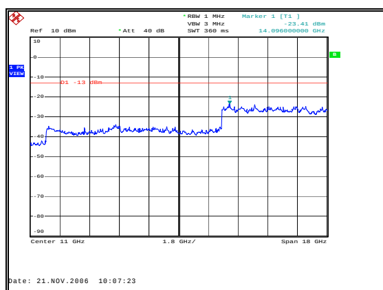
Figure 49: Spurious Emissions-Downlink CDMA Low Channel–Inter-modulation-2 GHz to 20 GHz
