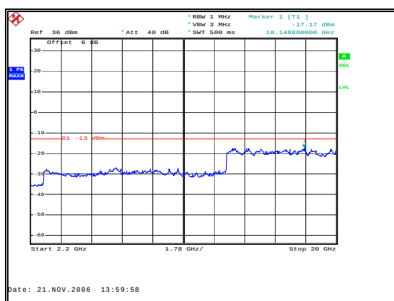
Figure 23: Spurious Emissions - Uplink CDMA Mid Channel – 2.2 GHz to 20 GHz
