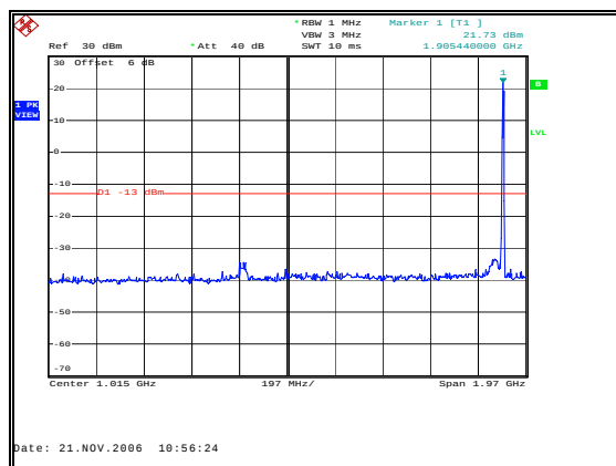
Figure 25: Spurious Emissions - Uplink CDMA High Channel-Inter-modulation-30 MHz to 2 GHz
