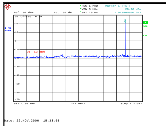
Figure 45: Spurious Emissions - Uplink GSM High Channel – 30 MHz to 2.2 GHz
