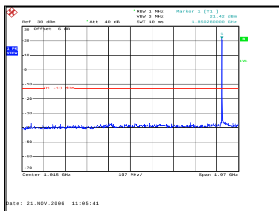
Figure 28: Spurious Emissions - Uplink TDMA Low Channel – Inter-modulation-30 MHz to 2 GHz
