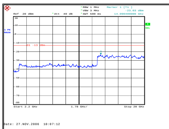
Figure 59: Spurious Emissions - Downlink TDMA Mid Channel – 2.2 GHz to 20 GHz
