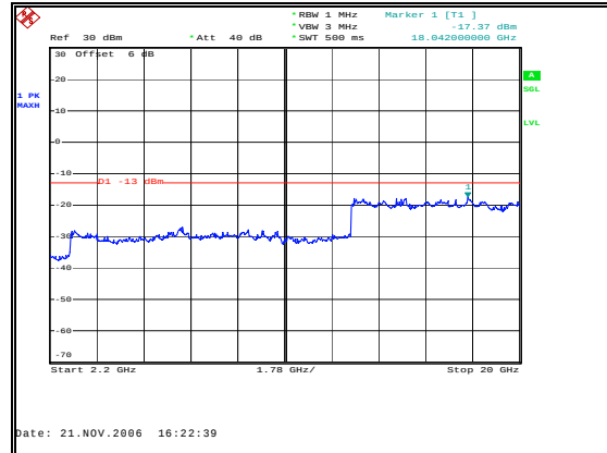
Figure 44: Spurious Emissions - Uplink GSM Mid Channel – 2.2 GHz to 20 GHz
