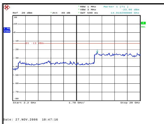
Figure 74: Spurious Emissions - Downlink GSM High Channel – 2.2 GHz to 20 GHz
