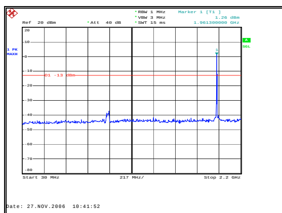
Figure 71: Spurious Emissions - Downlink GSM Mid Channel – 30 MHz to 2.2 GHz
