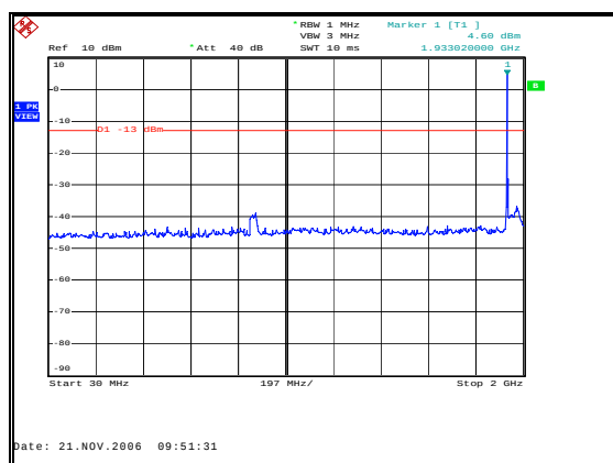
Figure 56: Spurious Emissions-Downlink TDMA Low Channel–Inter-modulation-30MHz to 2GHz
