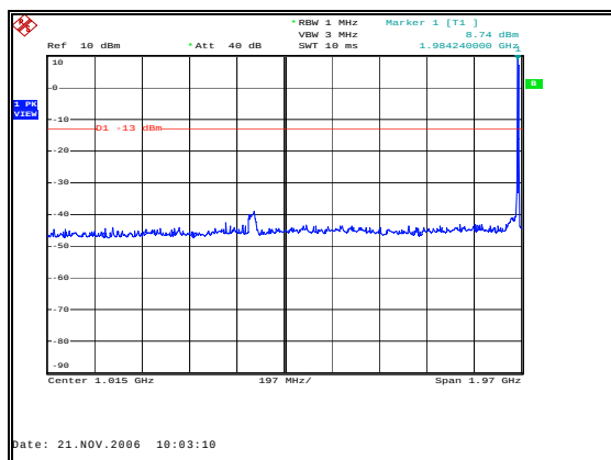
Figure 53: Spurious Emissions-Downlink CDMA High Channel-Inter-modulation-30MHz to 2GHz
