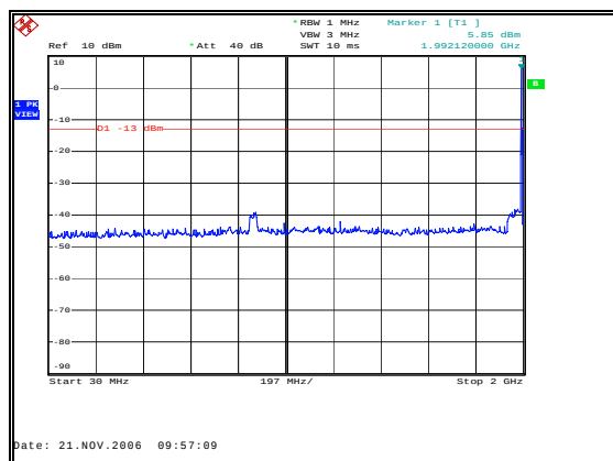
Figure 61: Spurious Emissions-Downlink TDMA High Channel-Inter-modulation-30MHz to 2GHz
