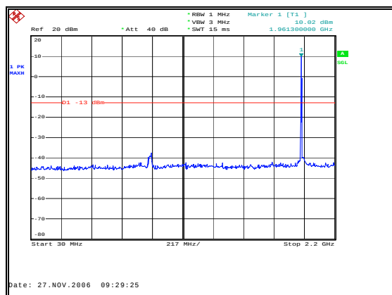
Figure 50: Spurious Emissions - Downlink CDMA Mid Channel – 30 MHz to 2.2 GHz
