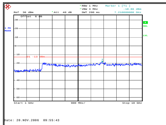
Figure 23: Spurious Emissions - Uplink CDMA Mid Channel – 1 to 10 GHz
