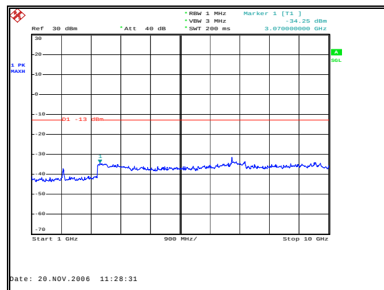
Figure 51: Spurious Emissions - Downlink CDMA Mid Channel – 1 to 10 GHz
