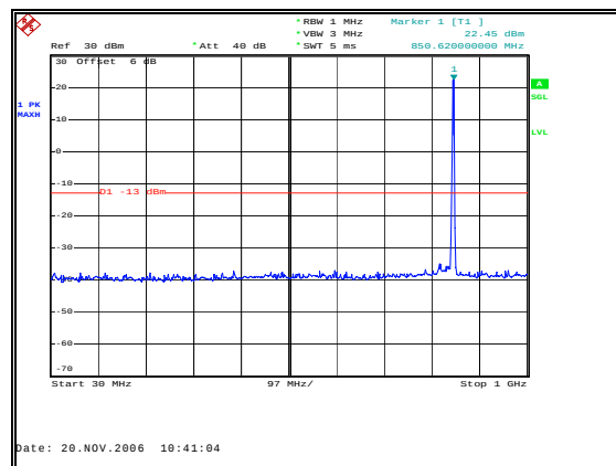
Figure 45: Spurious Emissions - Uplink GSM High Channel – 30 MHz to 1 GHz
