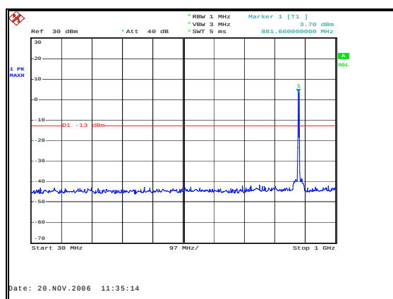
Figure 71: Spurious Emissions - Downlink GSM Mid Channel – 30 MHz to 1 GHz
