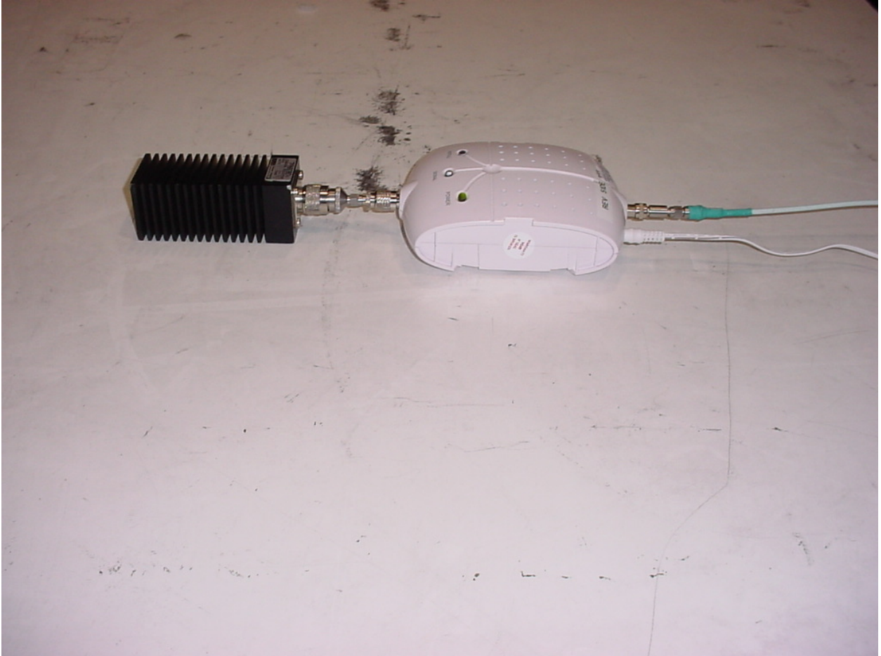
Figure 2: Test Setup – Intentional Spurious Emissions
