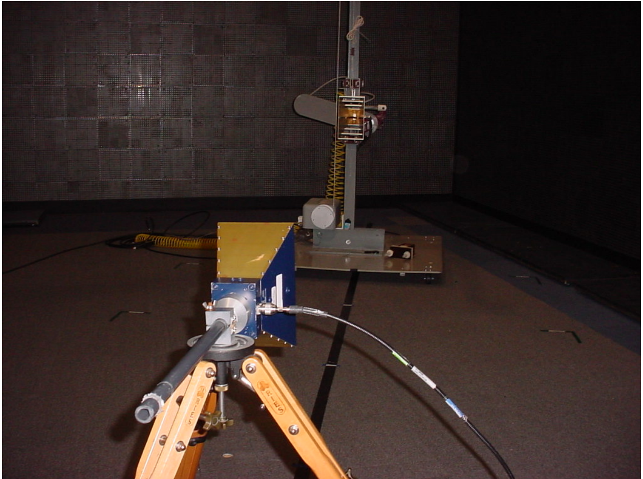
Figure 3: Test Setup – Intentional Spurious Emissions - Substitution
