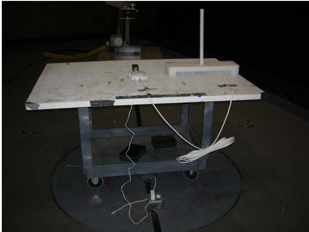
Figure 4: Test Setup – Unintentional Radiated Emissions
