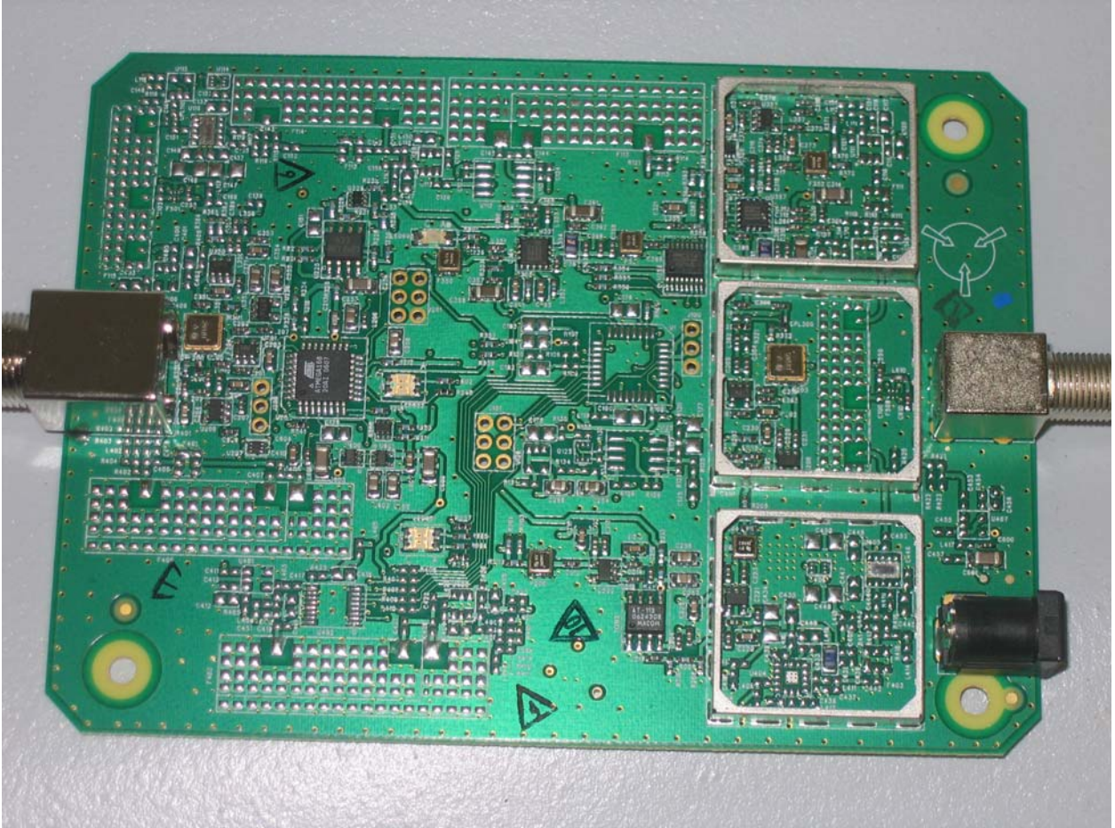
Figure 2: Internal – PCB Front – Unshielded
