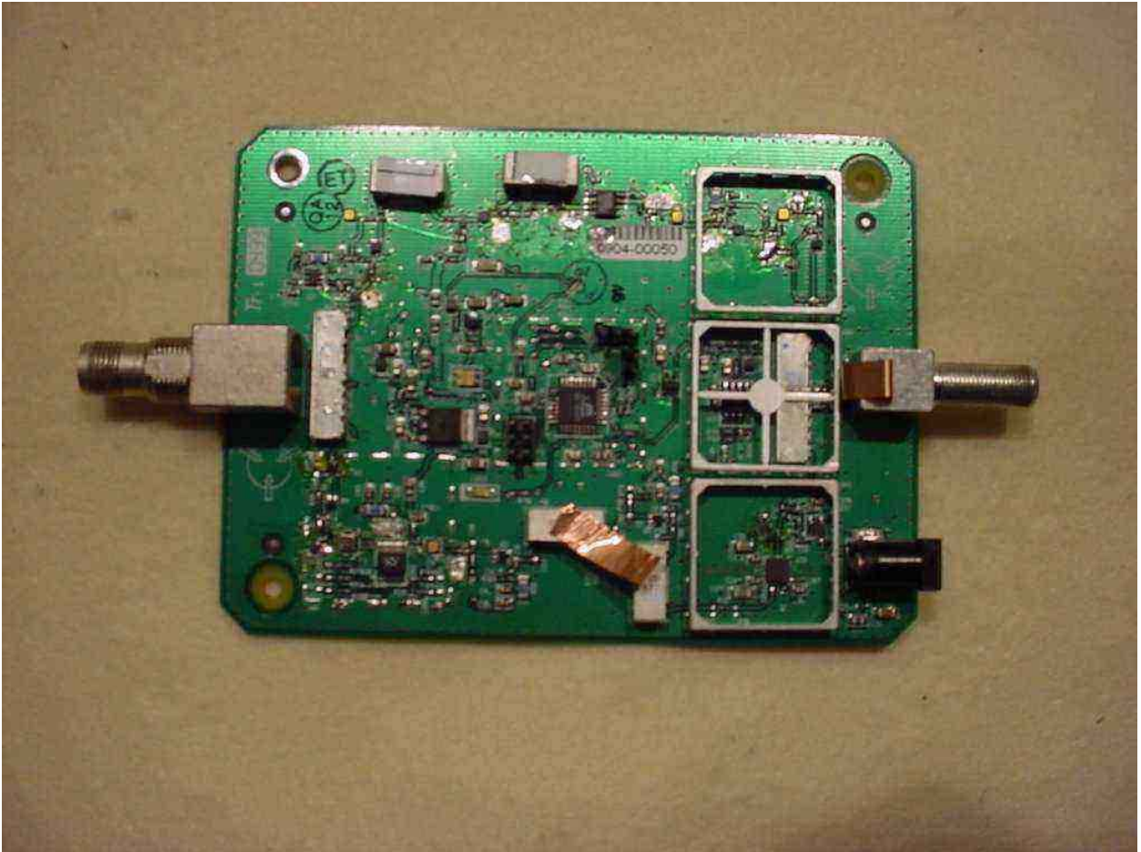
Figure 2: EUT PCB Top View Shields Removed
