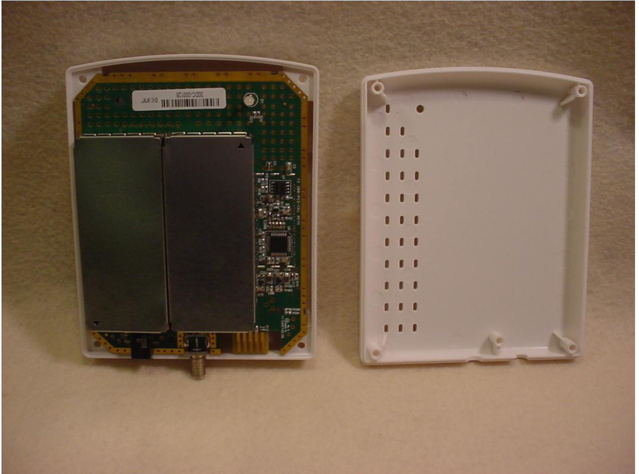
Figure 1: PCB Overview
