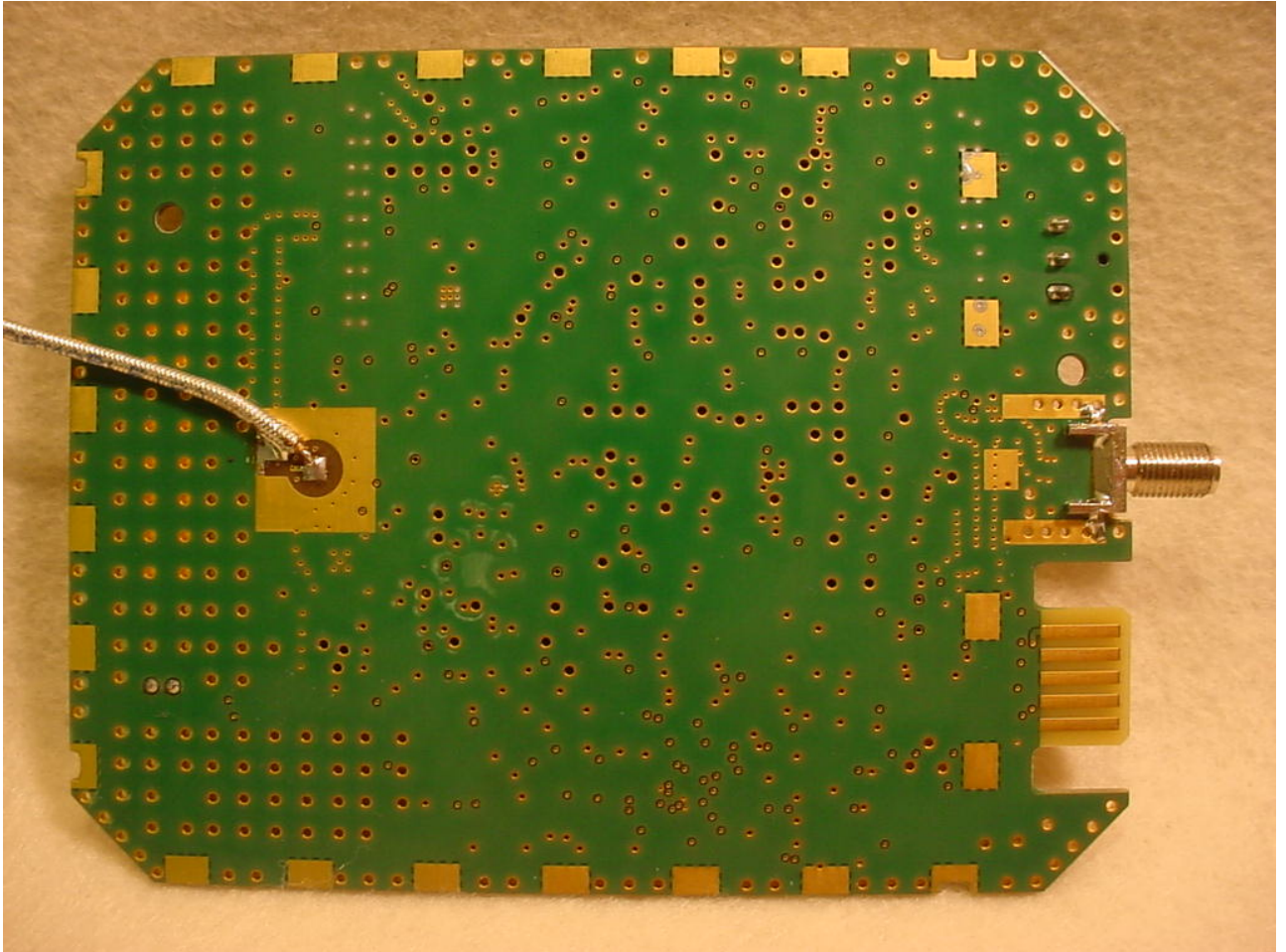
Figure 5: PCB Back – Without Antenna
