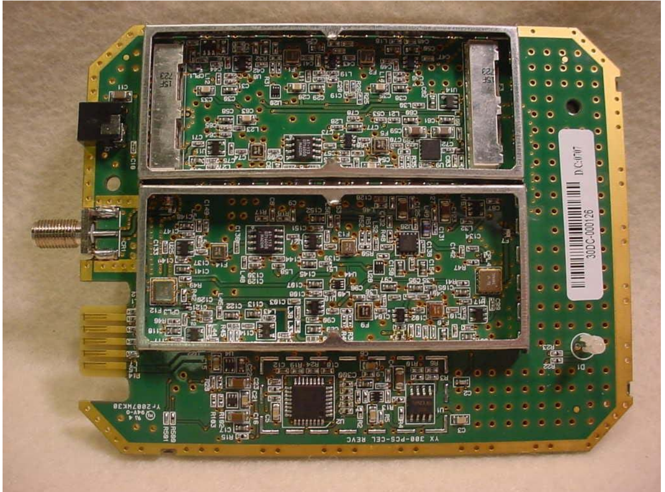
Figure 3: PCB Front – Without RF Shield
