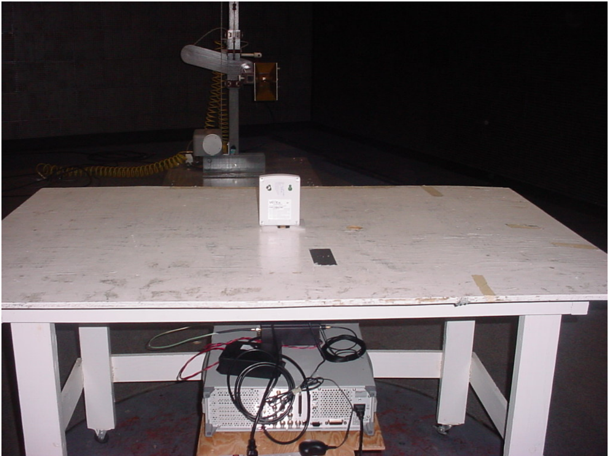
Figure 2: Radiated Emissions Test Setup - Uplink
