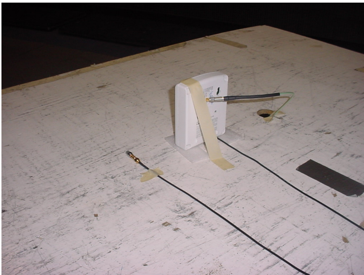
Figure 6: Radiated Emissions Test Setup Close Up – Downlink
