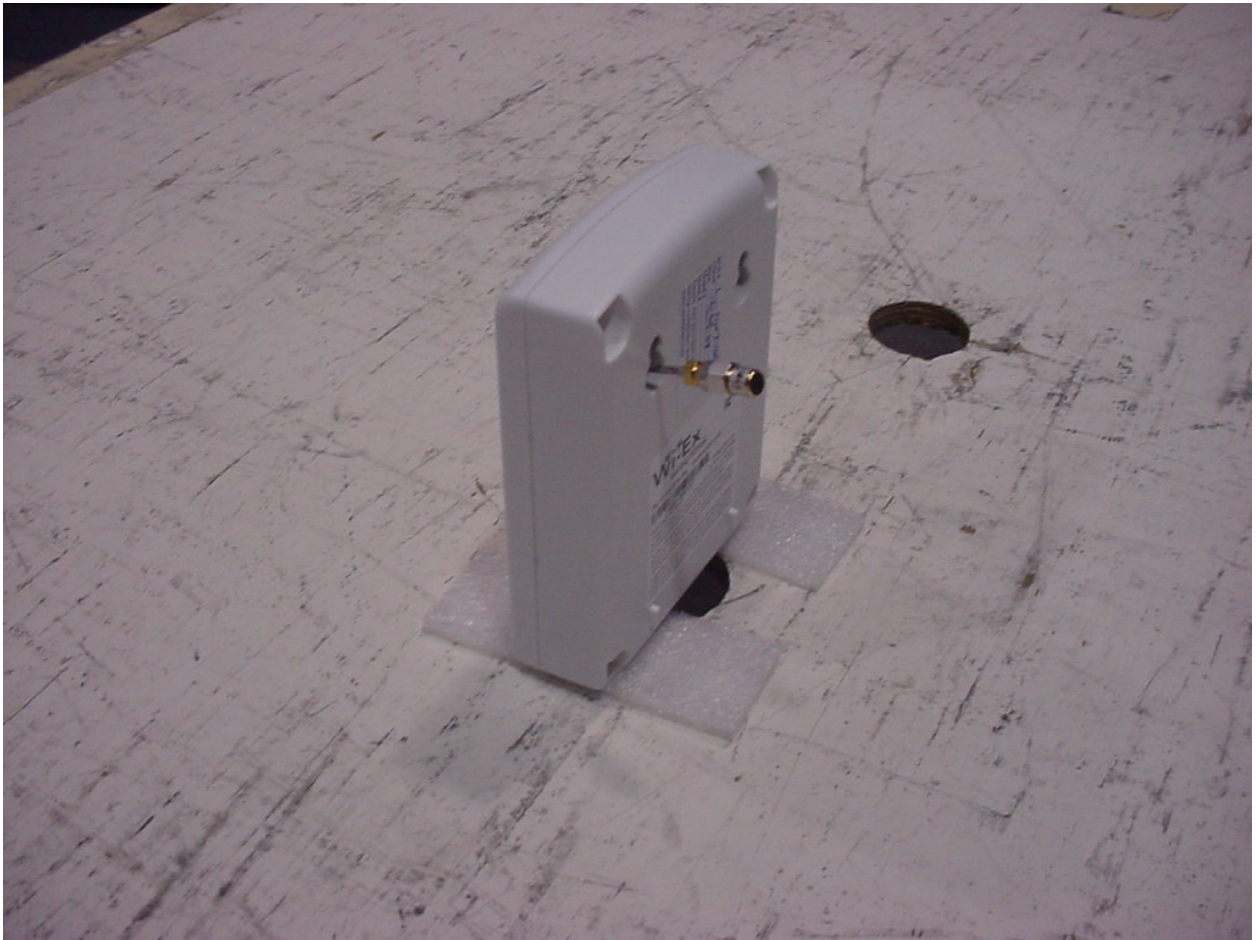
Figure 3: Radiated Emissions Test Setup Close Up – Uplink
