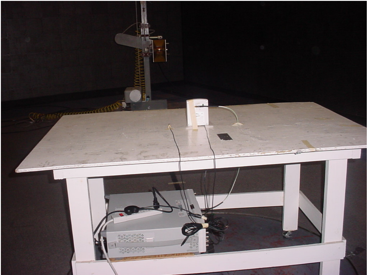
Figure 5: Radiated Emissions Test Setup – Downlink
