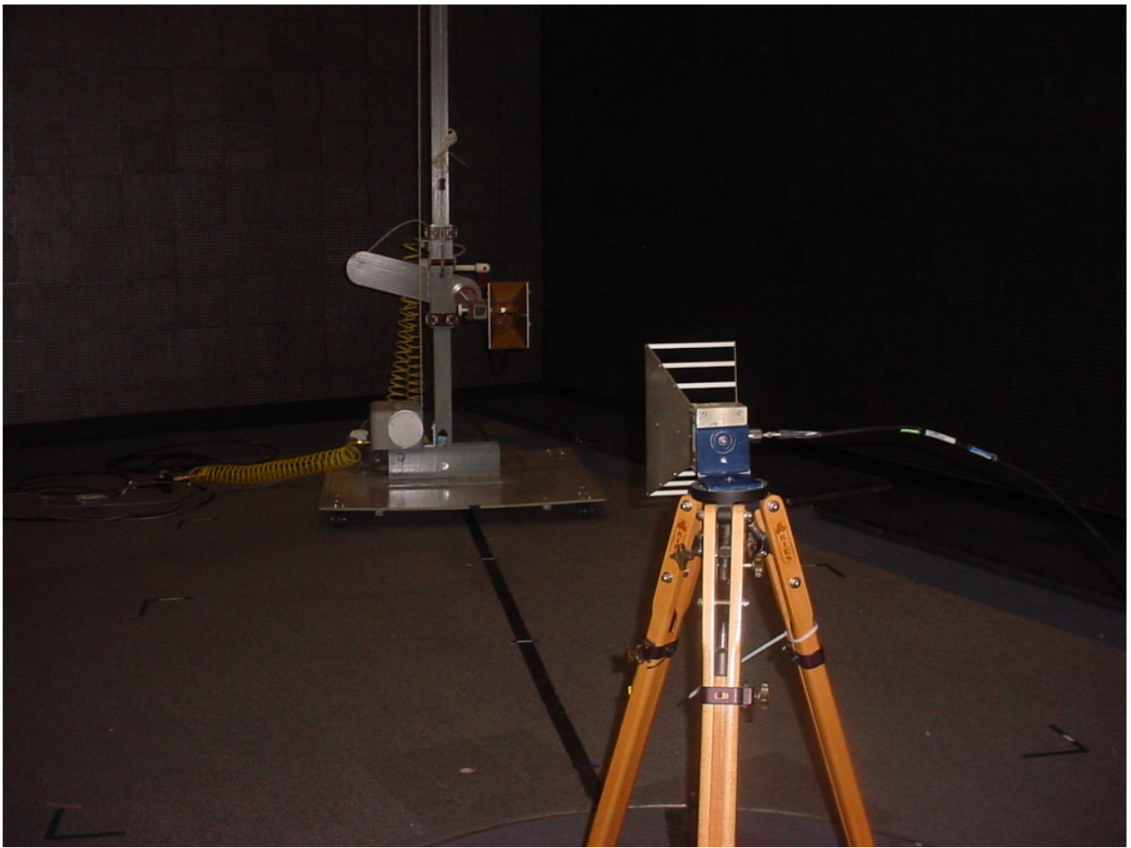
Figure 7: Radiated Emissions Test Setup – Substitution
