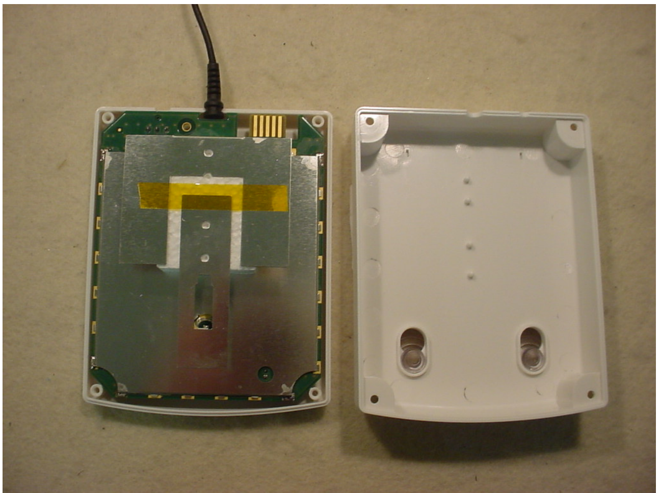
Figure 1: PCB Overview
