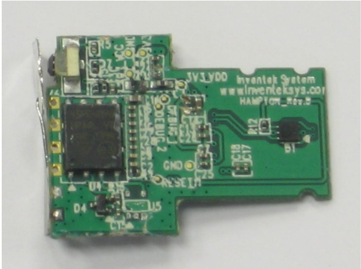
EUT internal photo, side 1
