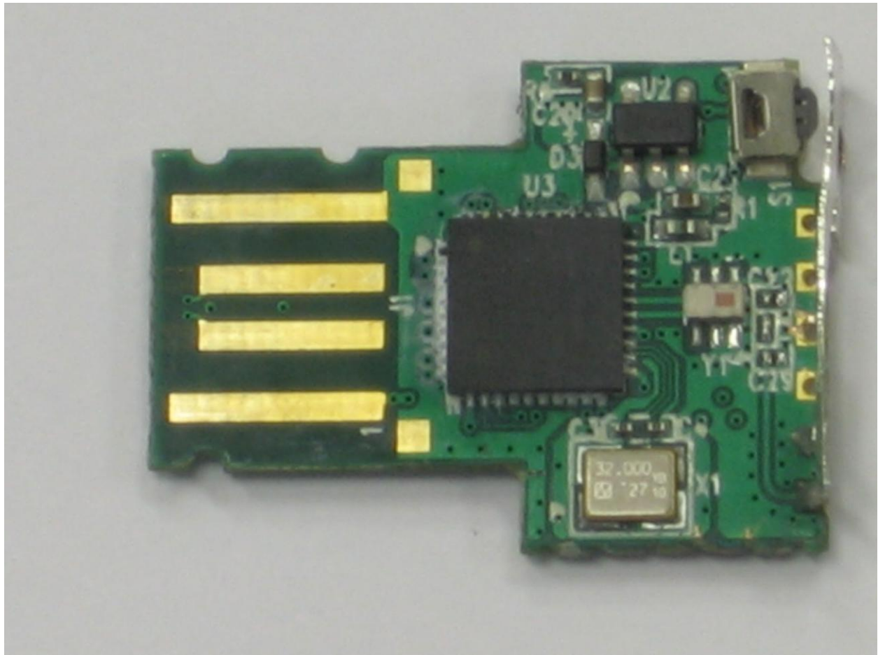
EUT internal photo, side 2
