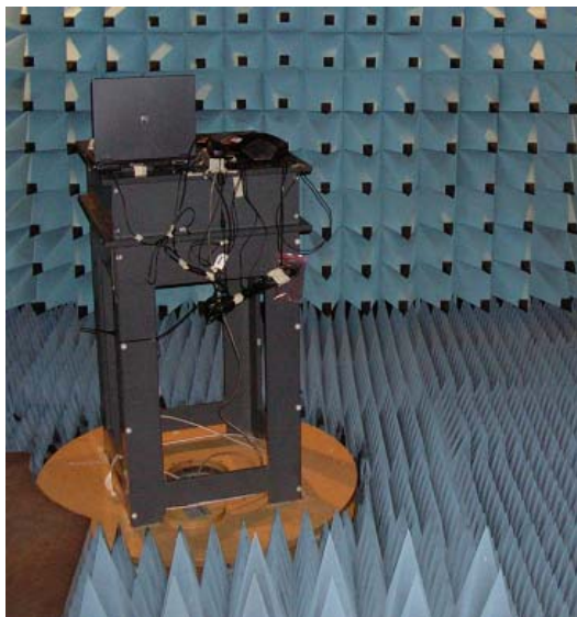
Spurious emission 1 – 10 GHz
