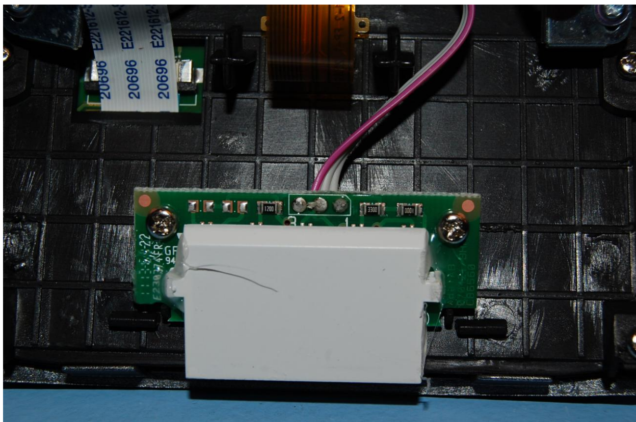
LED PCB with light guide
