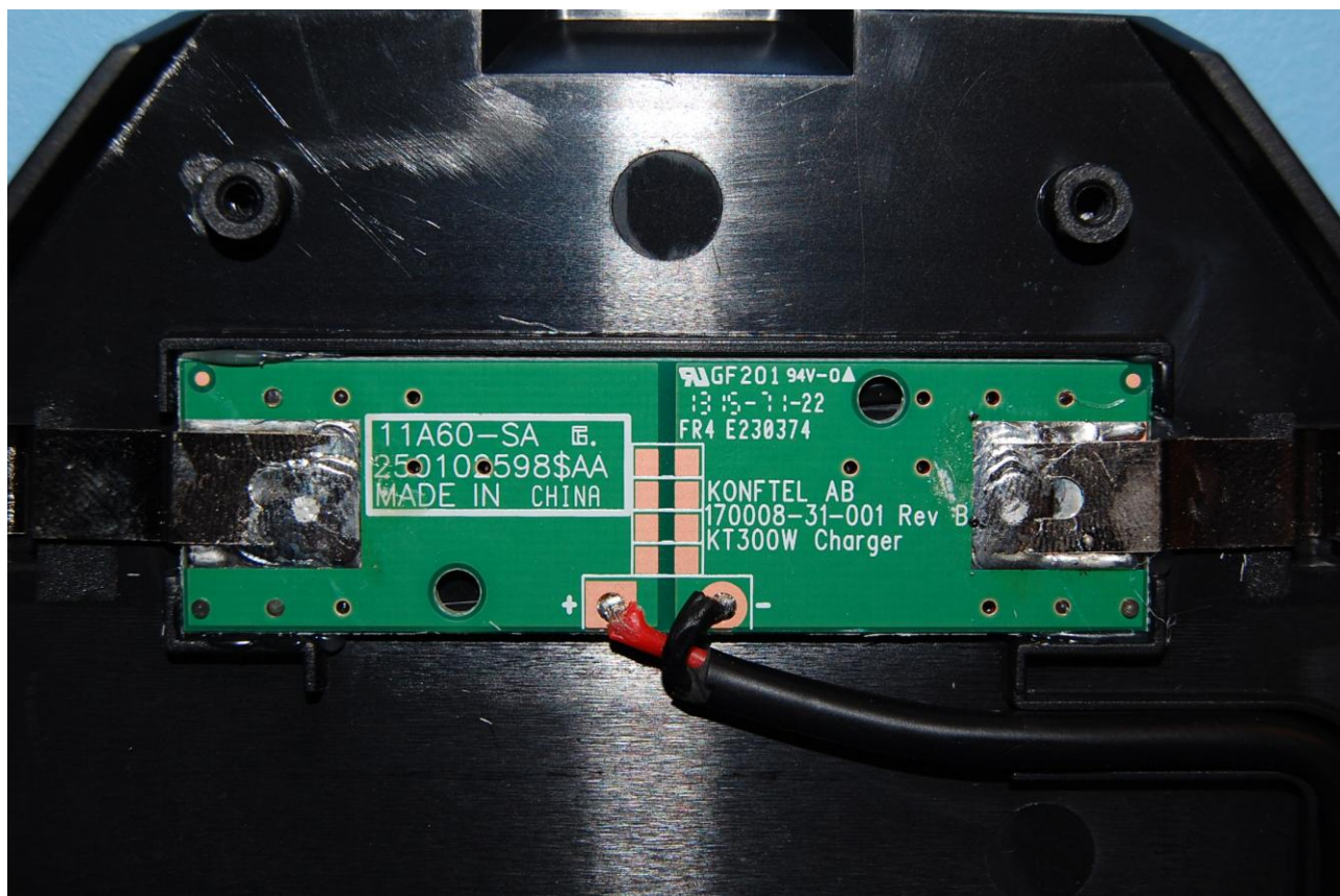
Charging cradle, internal PCB
