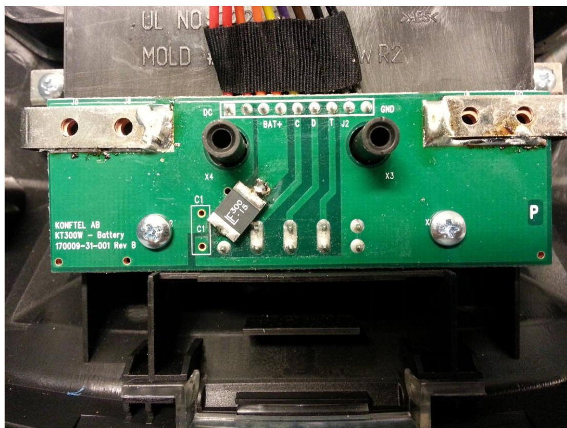
Battery PCB rear side
