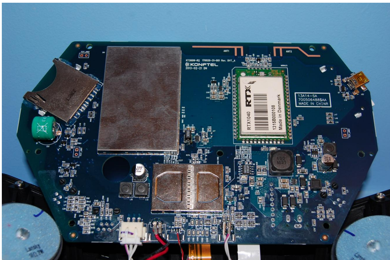
Main PCB, rear side
