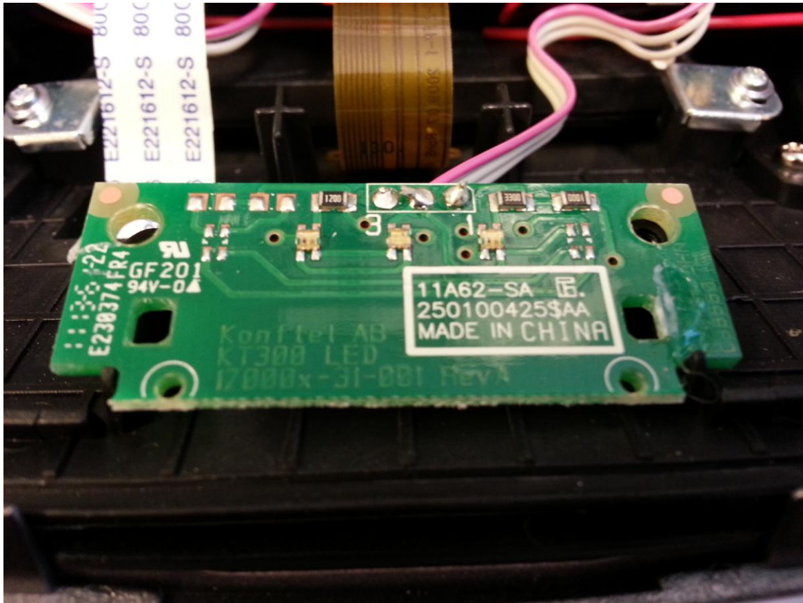
LED PCB top side, light guide removed
