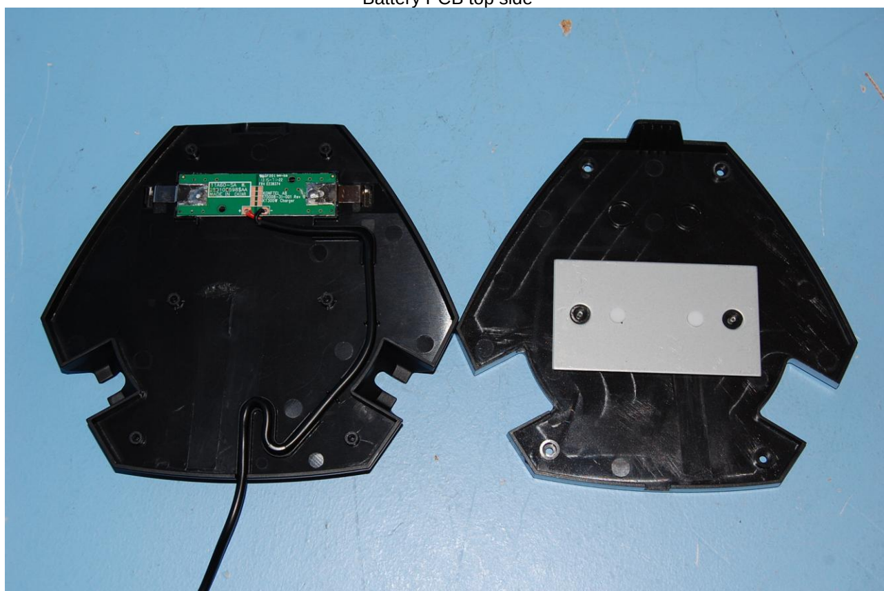
Charging cradle, internal view
