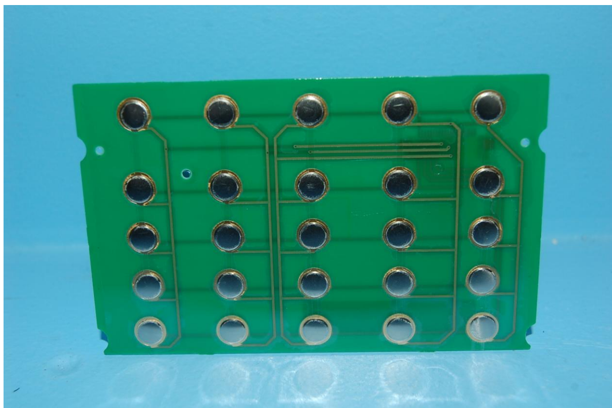
Keypad PCB rear side
