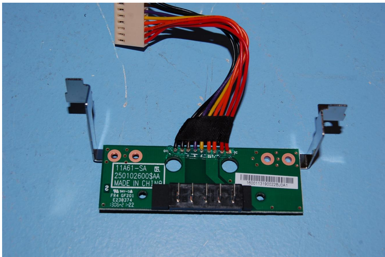
Battery PCB top side
