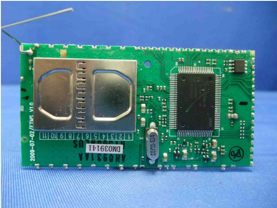
Conference Phone Unit Baseband and RF Module PCB comp side (View 1)
