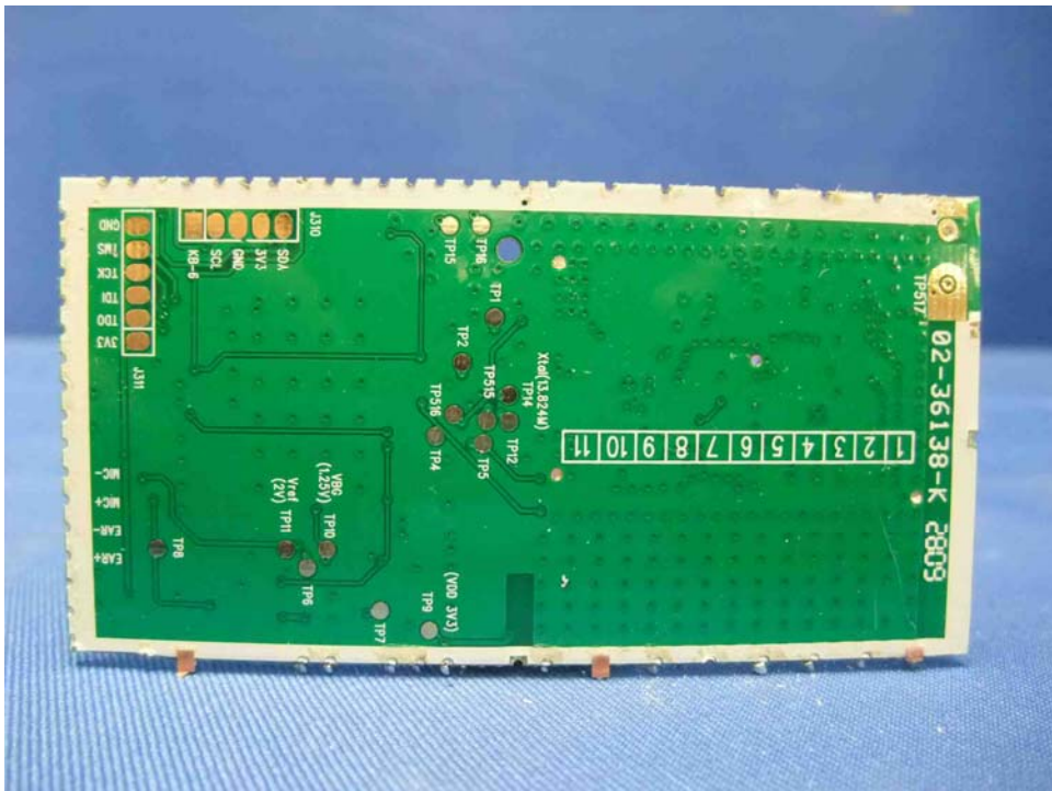
Conference Phone Unit Baseband and RF Module PCB solder side
