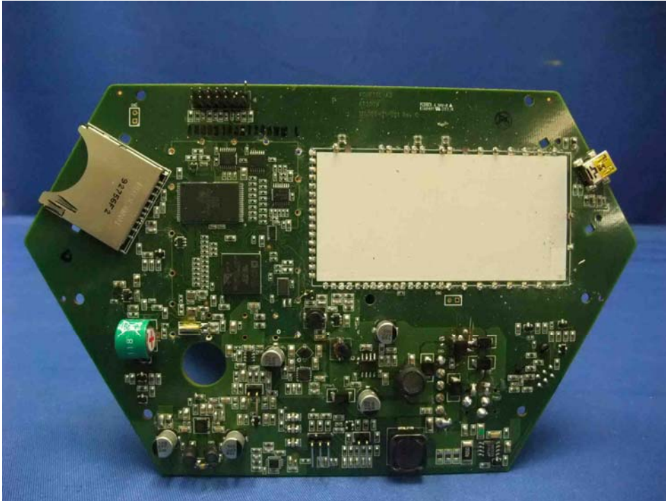
Conference Phone Unit Main PCB comp side (View 2)
