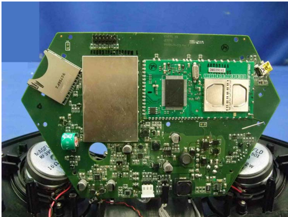
Conference Phone Unit Main PCB comp side (View 1)
