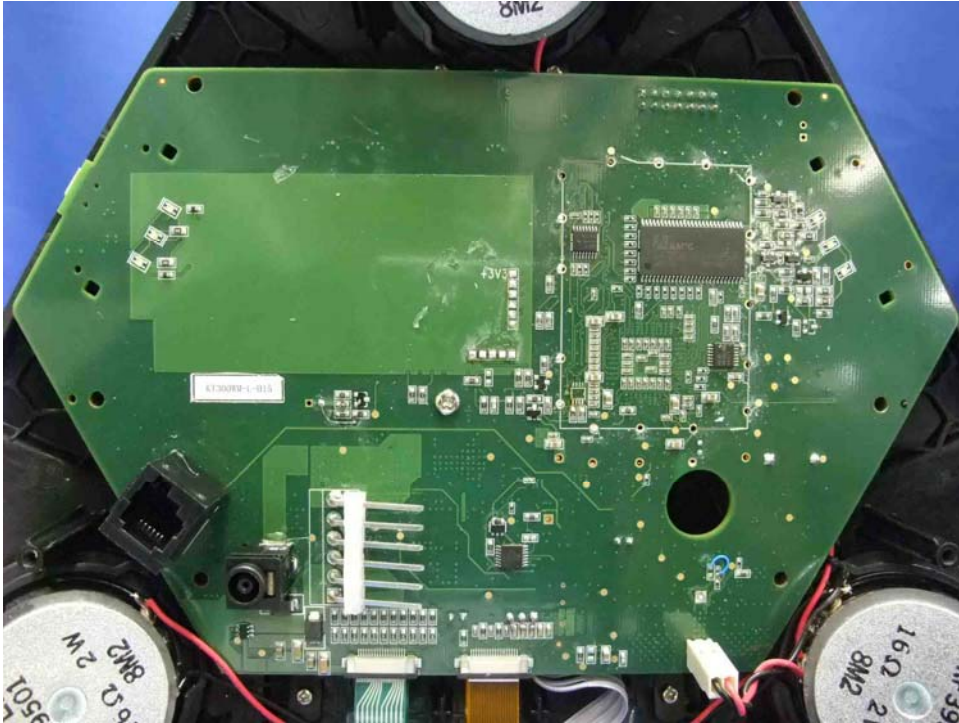
Conference Phone Unit Main PCB solder side (View 2)
