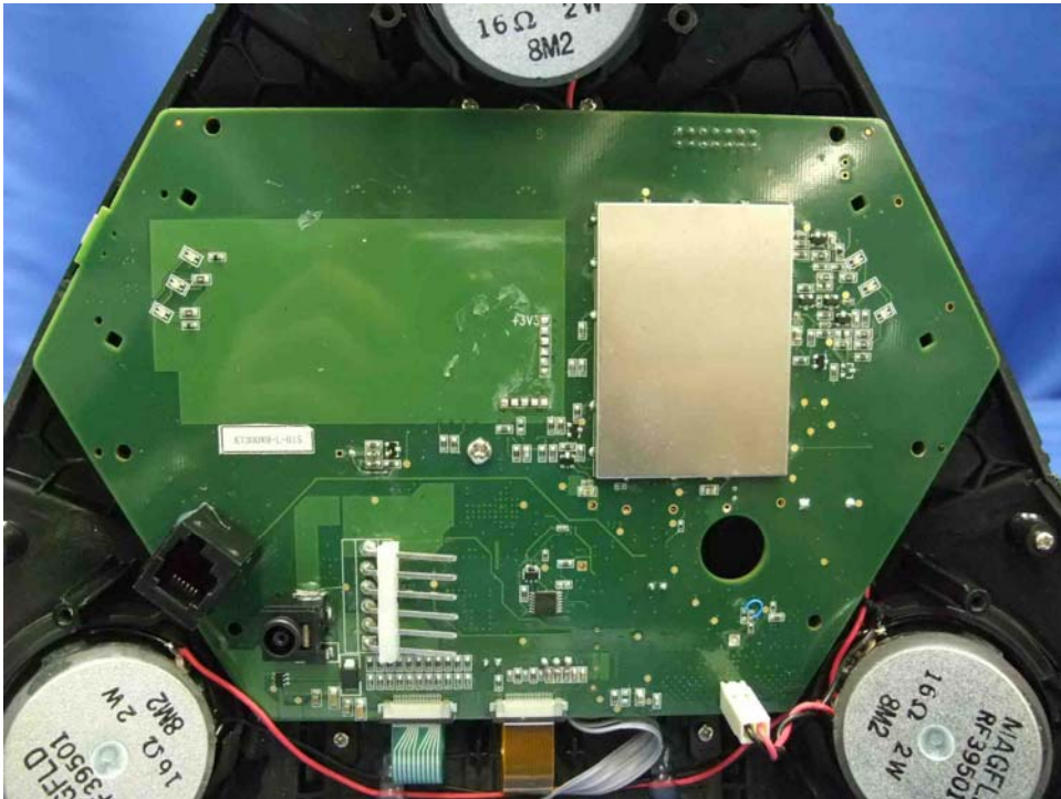
Conference Phone Unit Main PCB solder side (View 1)
