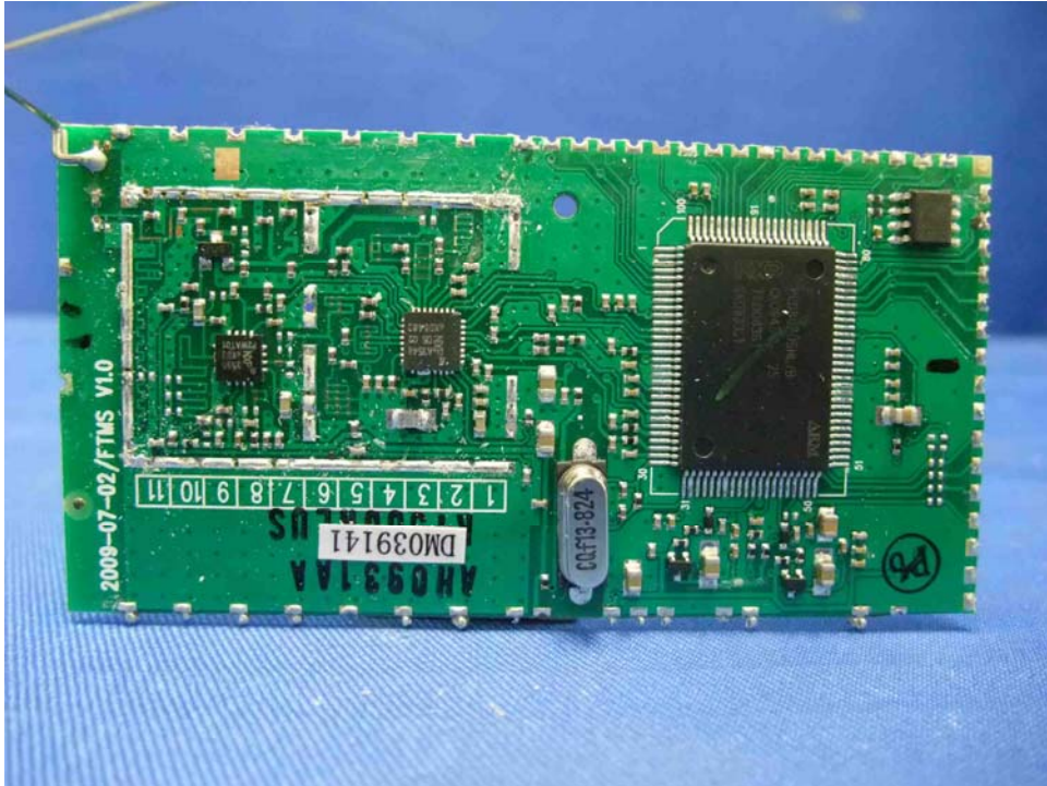
Conference Phone Unit Baseband and RF Module PCB comp side (View 2)
