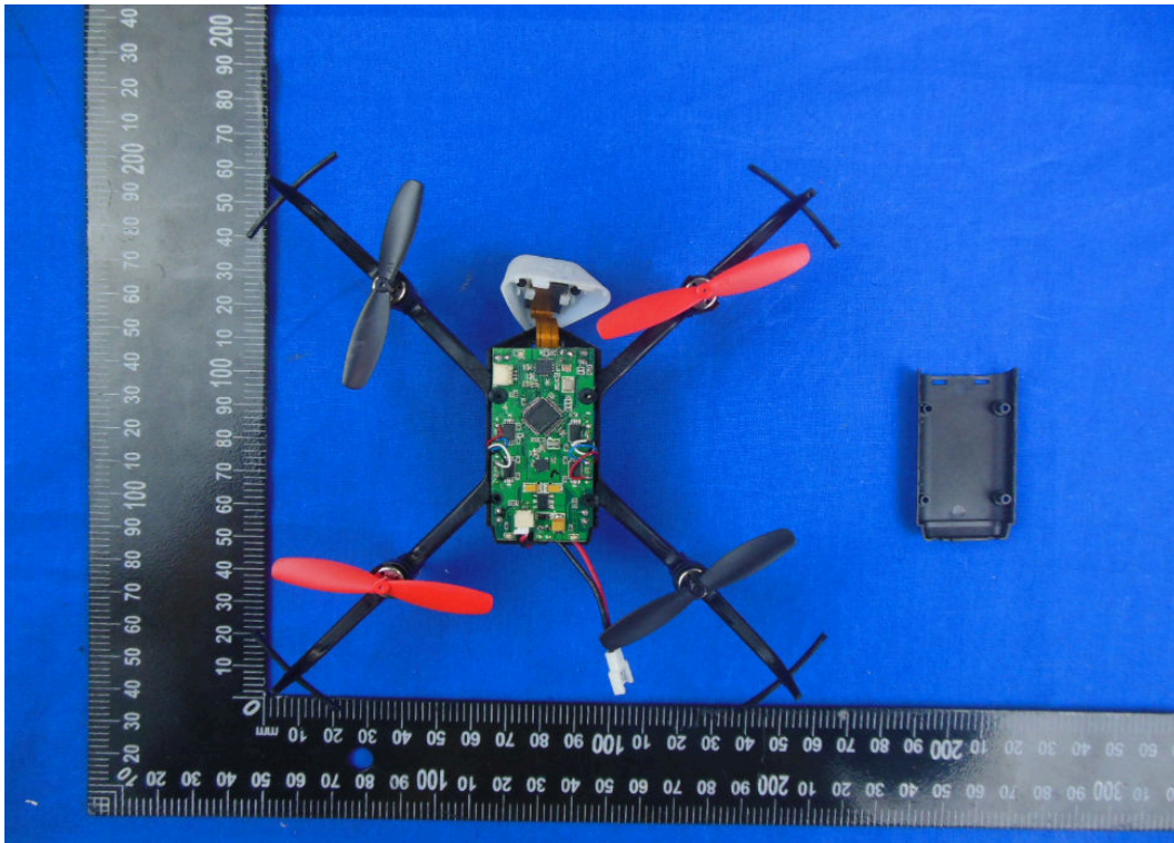
EUT - 2.4GHz PCB View
