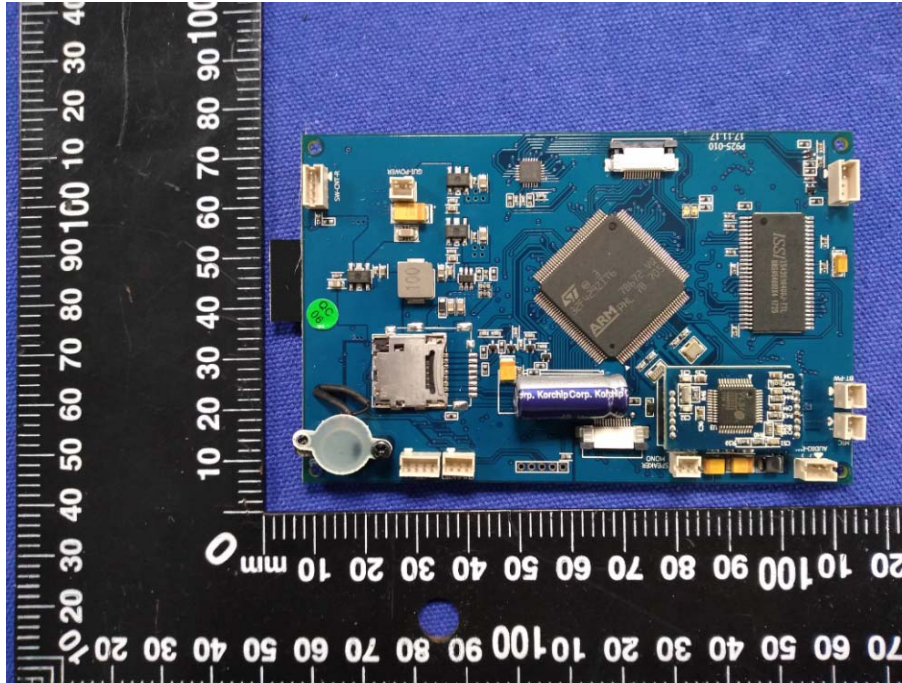
EUT – Main PCB View
