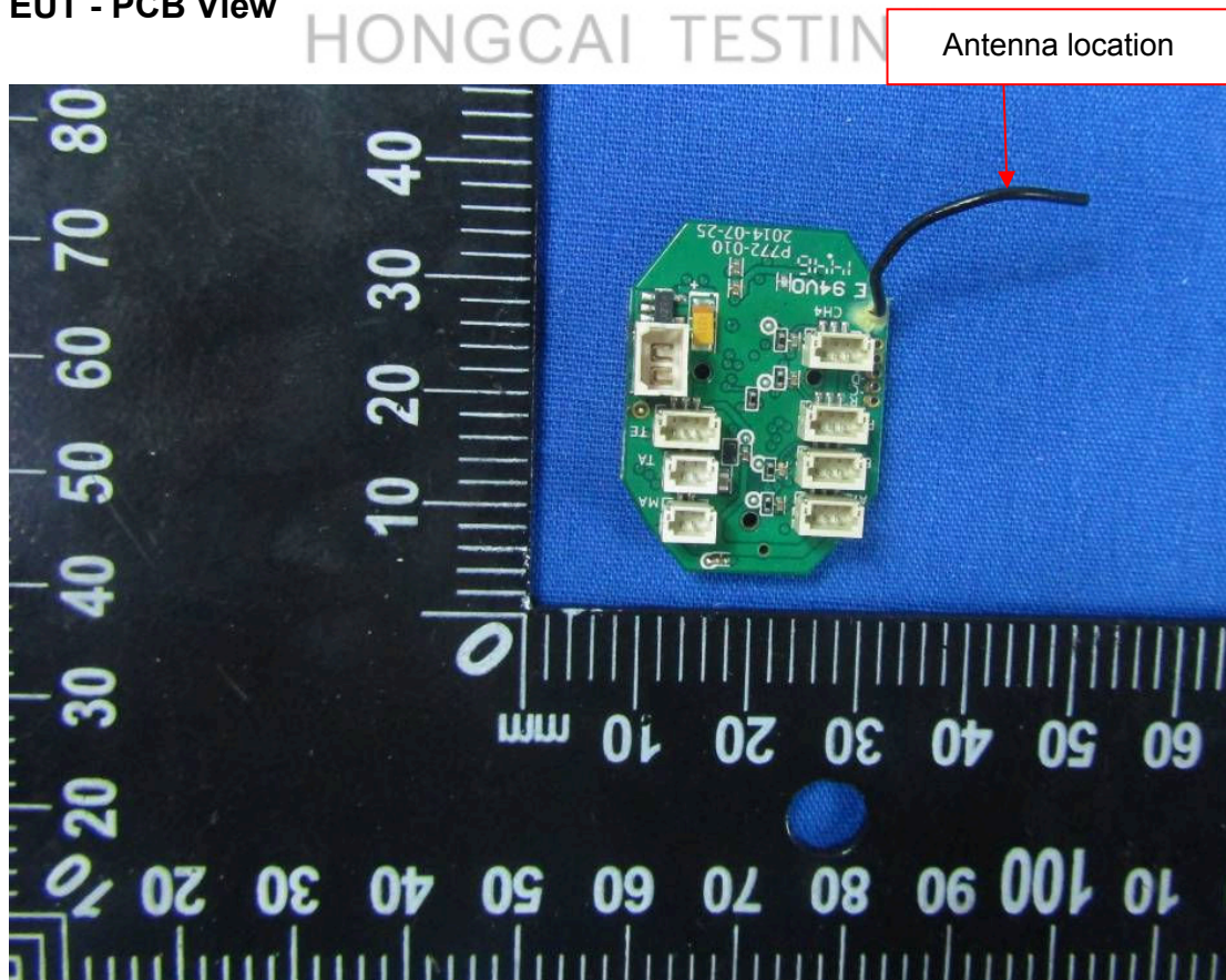
EUT - PCB View
