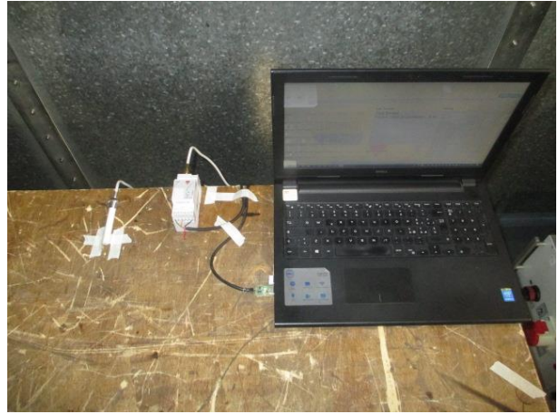
Radiated emissions (worst case orientation)
