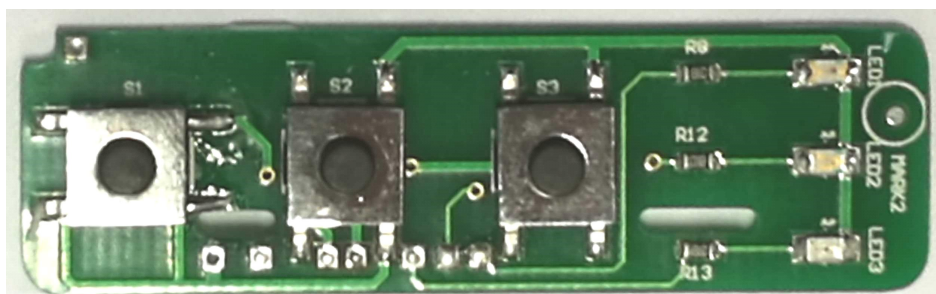
PCB CIC BLUETOOTH-3 – Top view
