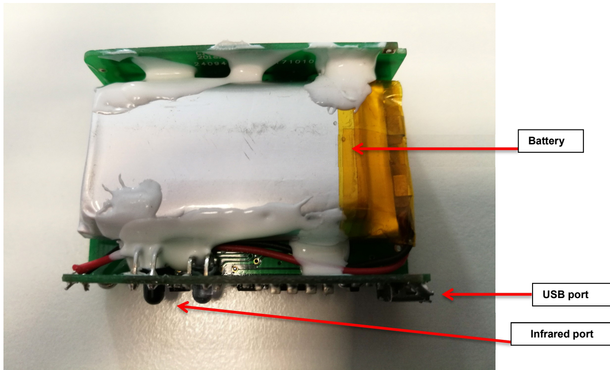
PCB CIC BLUETOOTH-1 – Bottom view (finished product)
