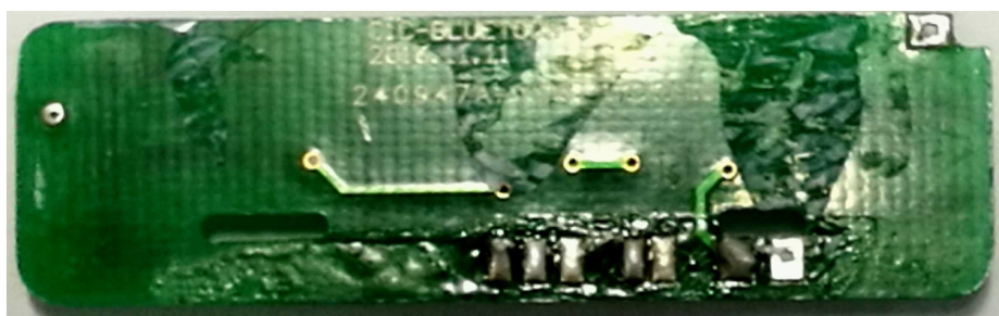
PCB CIC BLUETOOTH-3 – Bottom view
