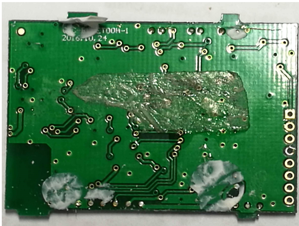
PCB CIC BLUETOOTH-1 – Bottom view (disassembled product)
