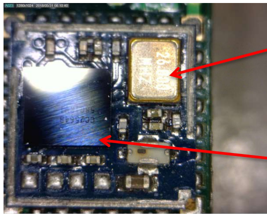
Details of Bluetooth® module without shield
