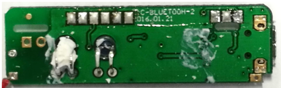
PCB CIC BLUETOOTH-2 – Bottom view
