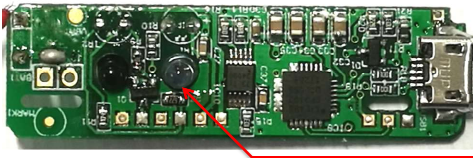
PCB CIC BLUETOOTH-2 – Top view
