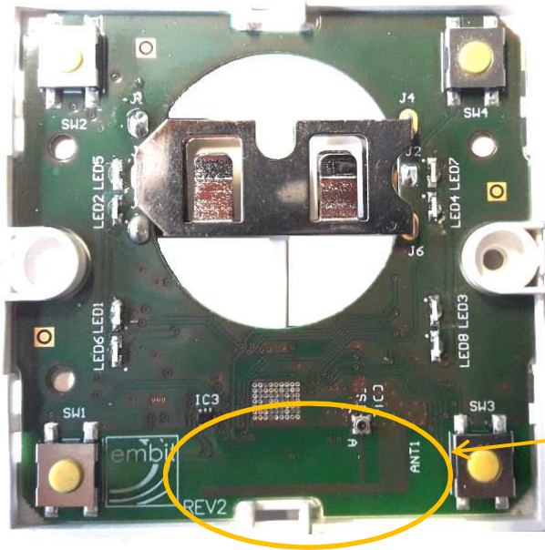
PCB removed from product, bottom view
