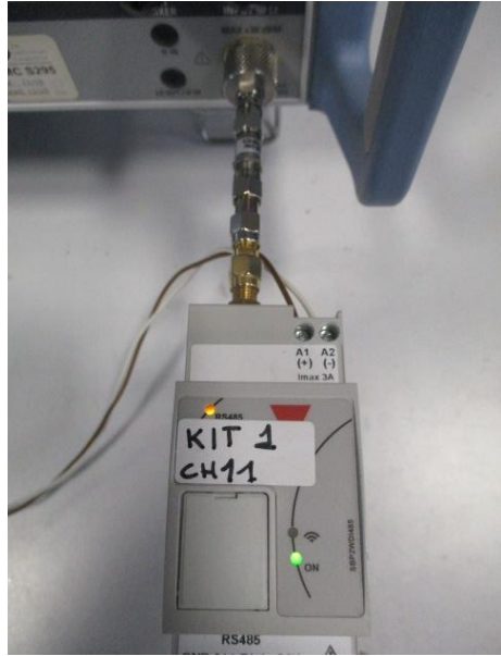
Conducted measurements on antenna port
