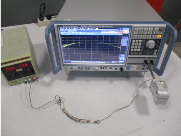
Conducted measurements on antenna port
