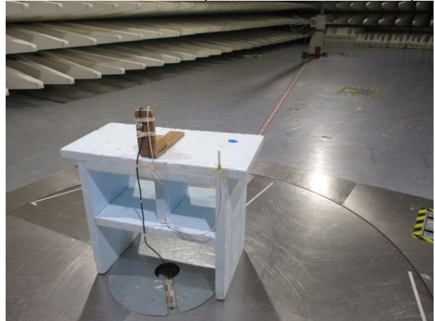
Radiated emissions (worst case orientation)
