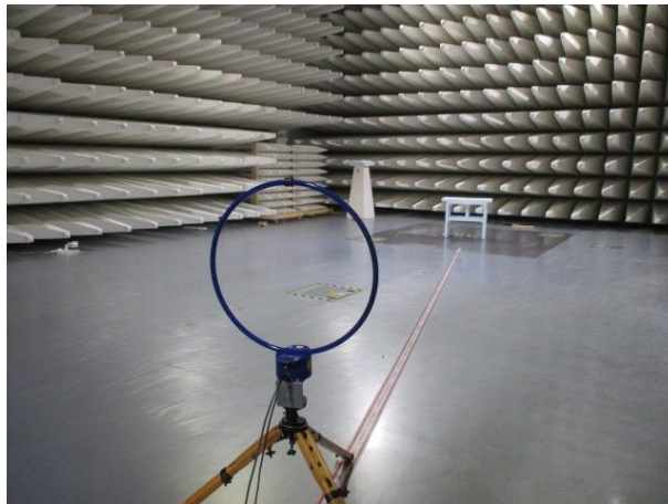
Radiated emissions
