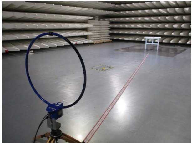
Radiated emissions
