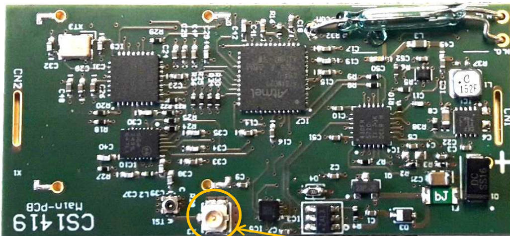
Antenna connector
