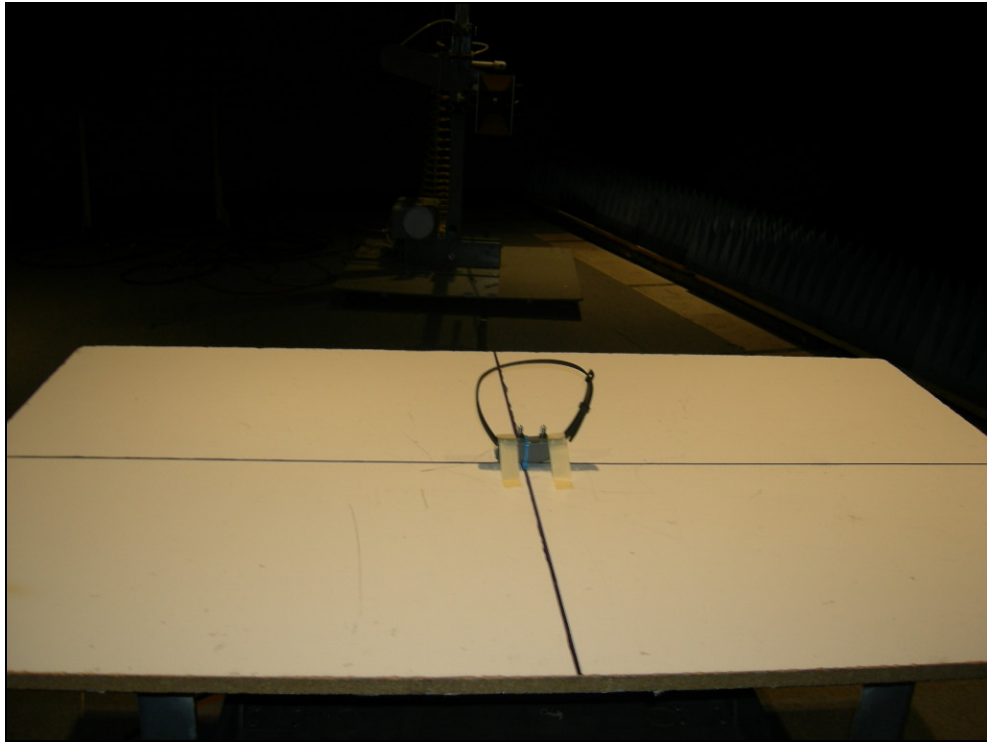
Figure 3: Radiated Emissions – Y Position
