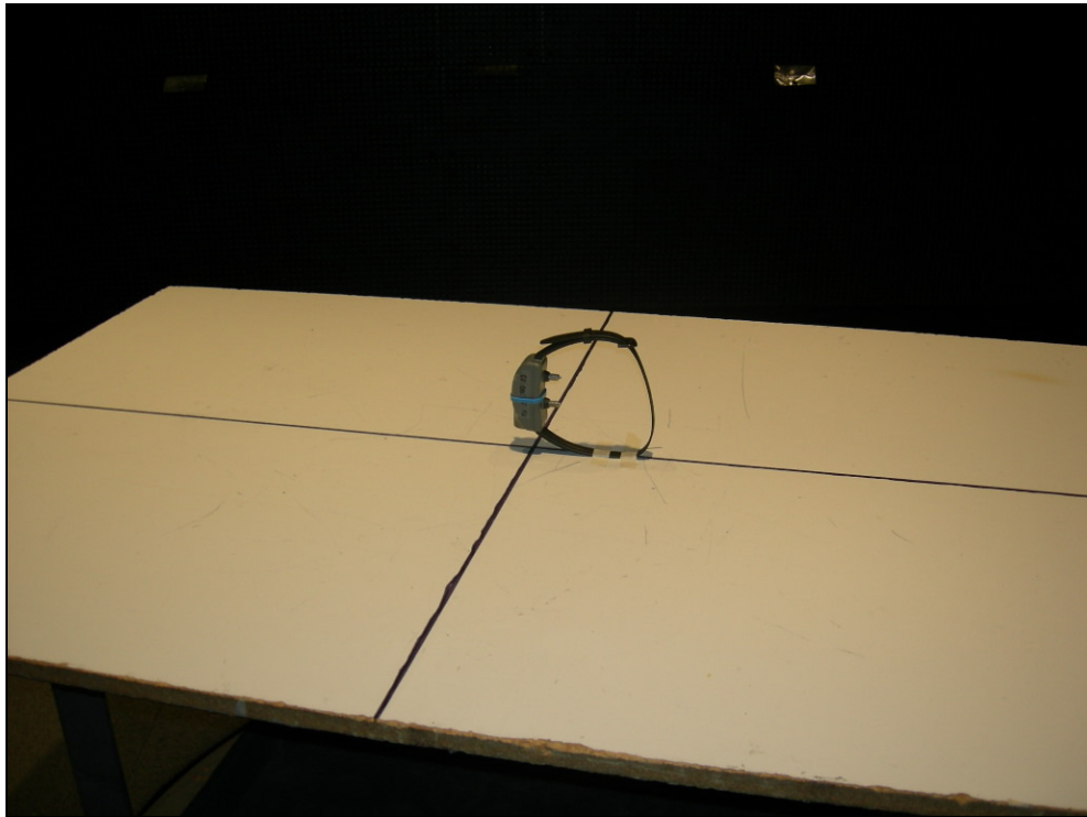
Figure 5: Radiated Emissions – Z Position
