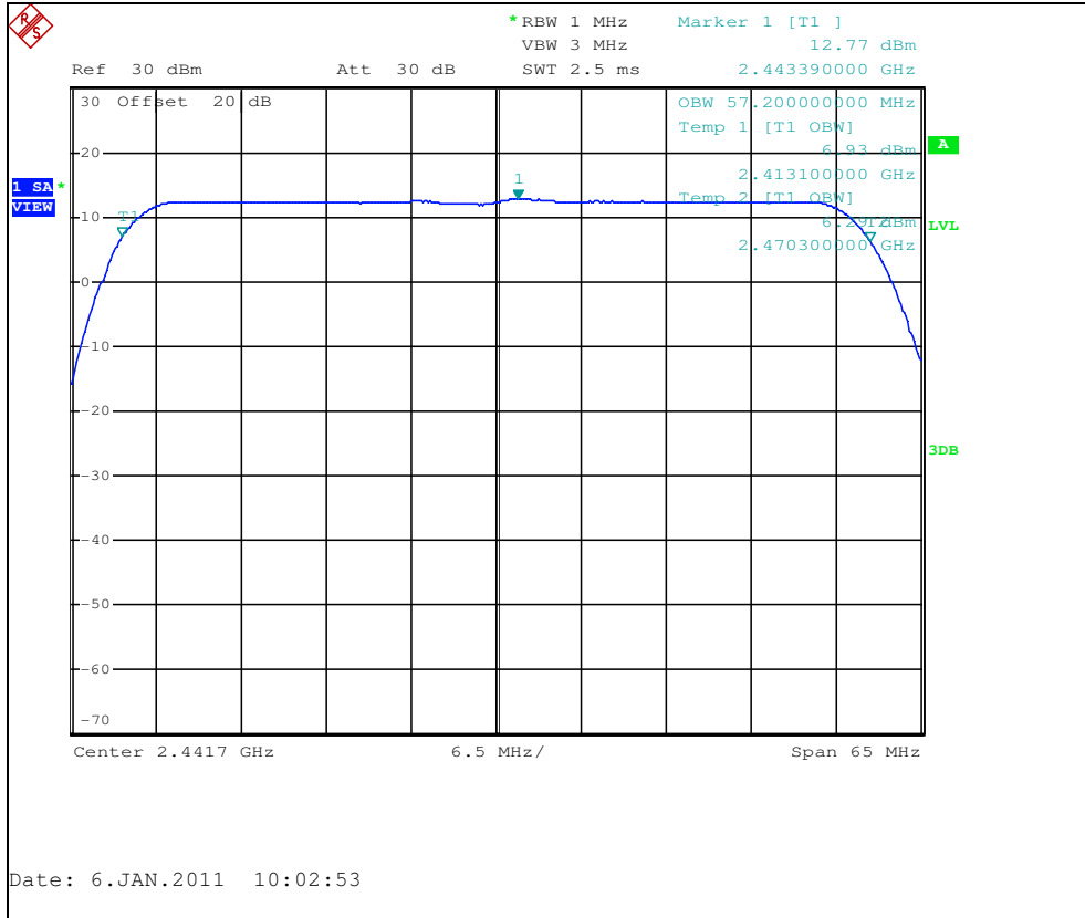
Figure 7.4.2-2: 99% Bandwidth Plot
