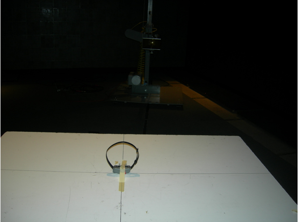
Figure 5: Radiated Emissions – Y Position
