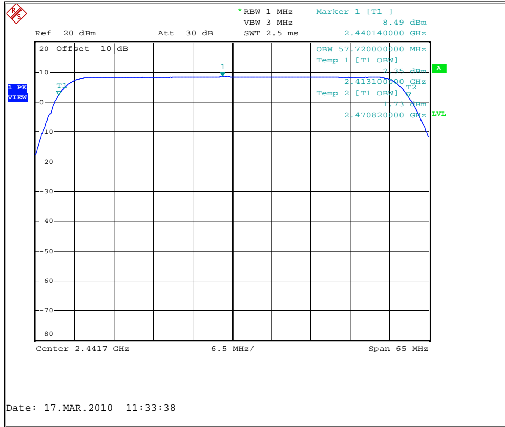
Figure 7.4.2-2: 99% Bandwidth Plot
