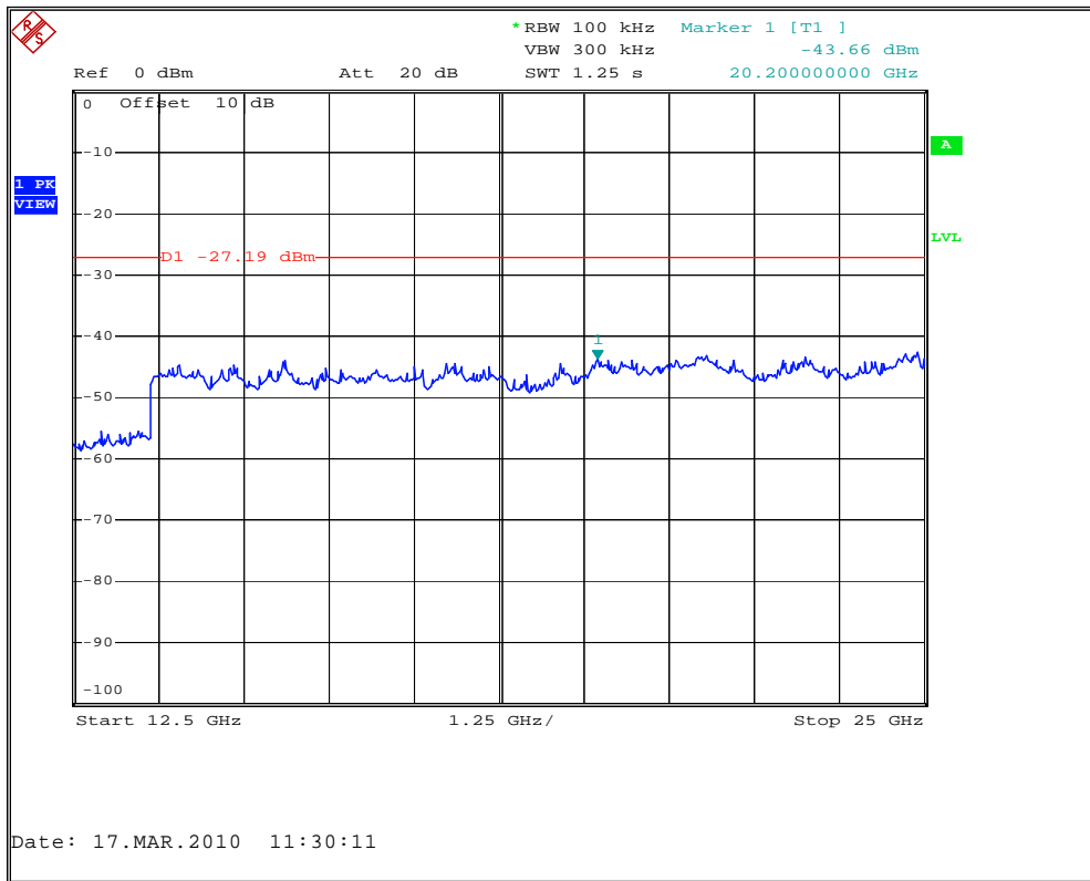
Figure 7.6.2.2-3: 12.5 GHz – 25 GHz
