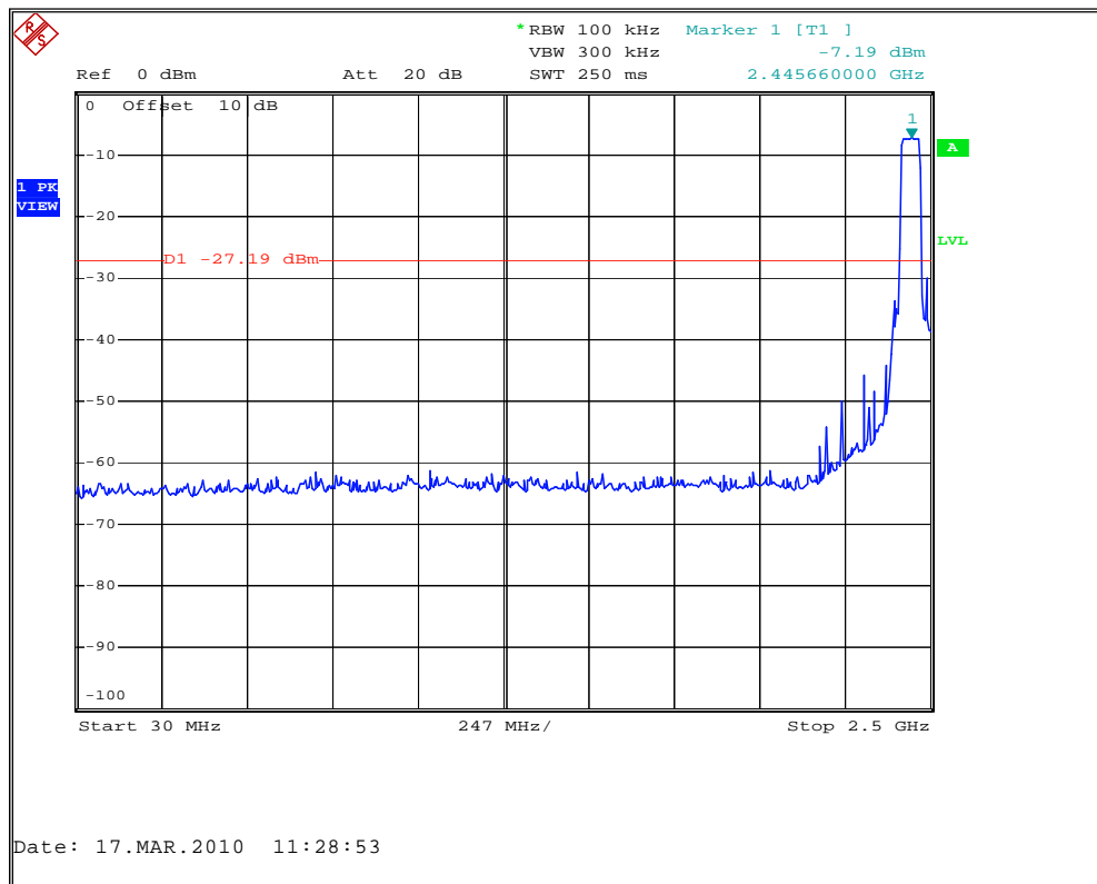
Figure 7.6.2.2-1: 30 MHz – 2.5 GHz
