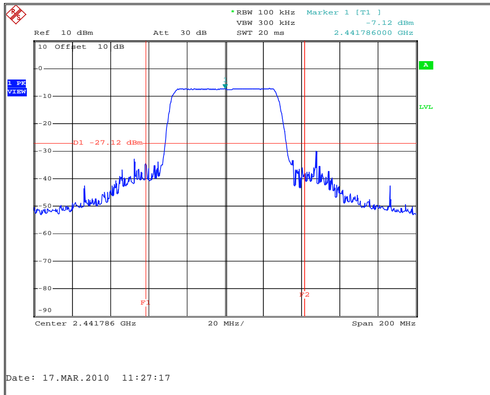
Figure 7.6.2.2-4: Band-edge (Conducted)
