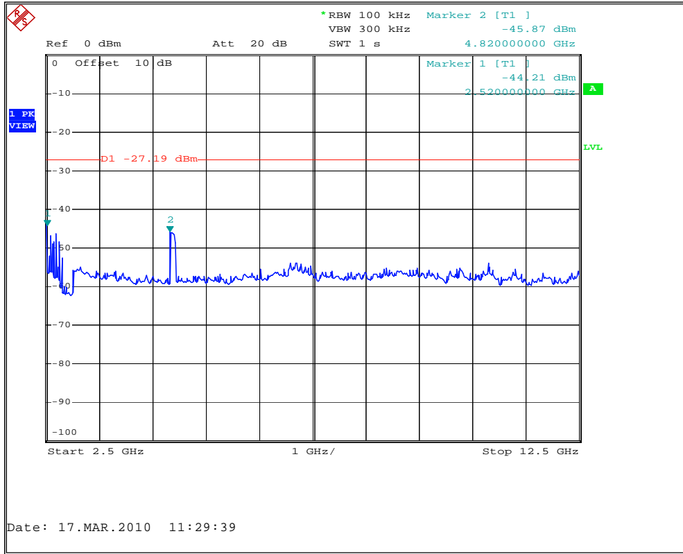
Figure 7.6.2.2-2: 2.5 GHz – 12.5 GHz
