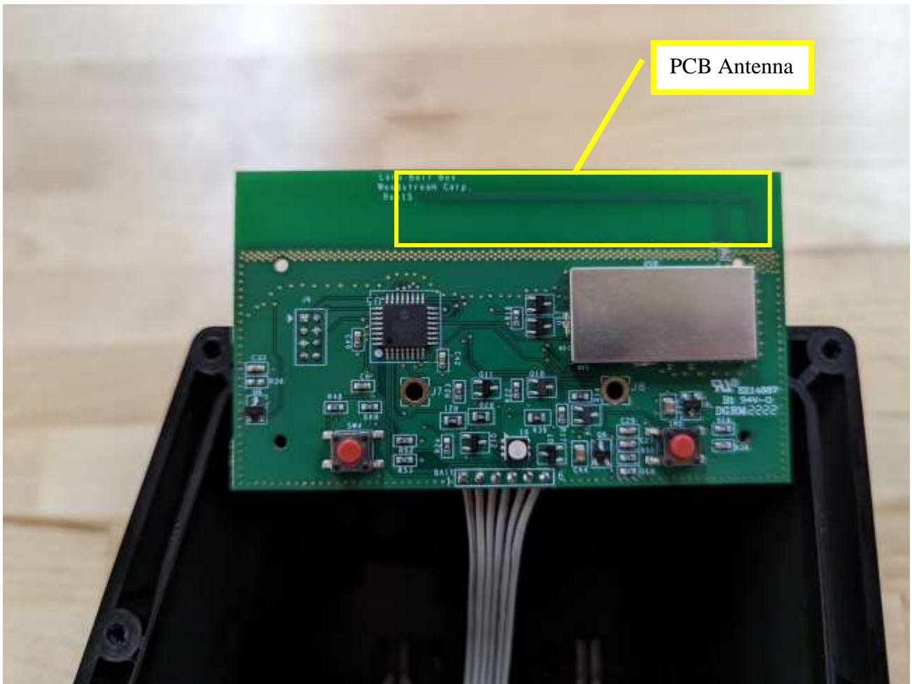
PCB Antenna Board With Shielding
