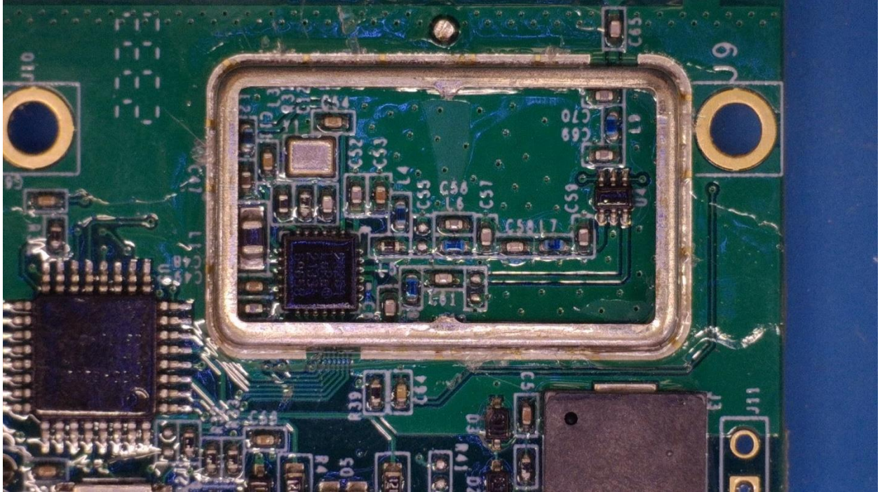
PCB Top Side Radio Close Up
