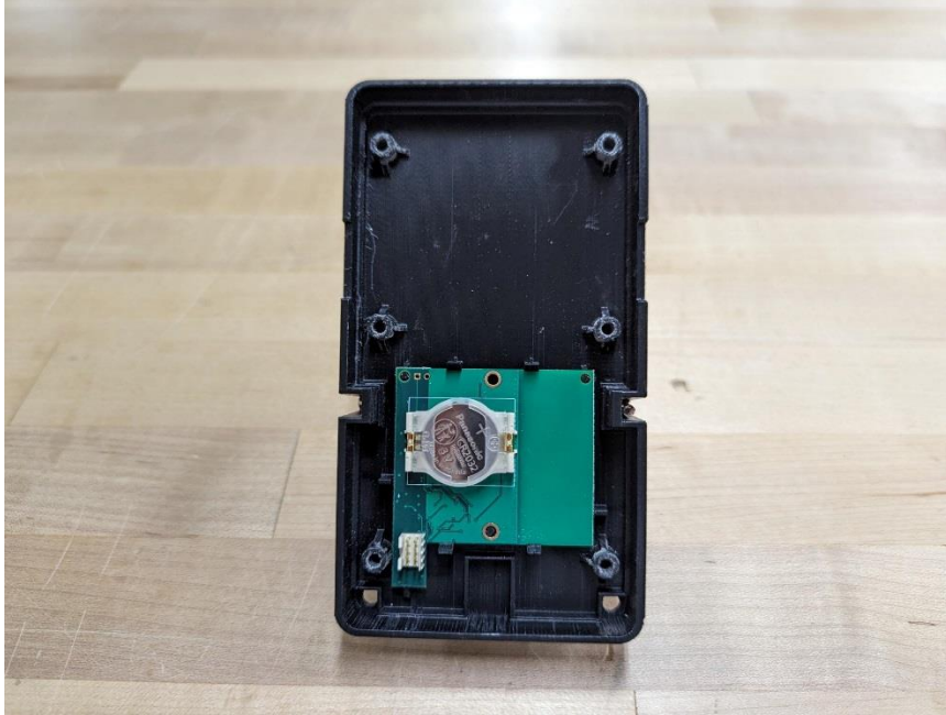
PCB Bottom Side with Battery
