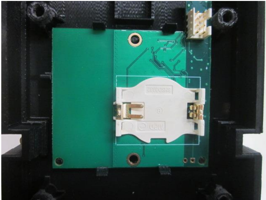
PCB Bottom Side without Battery
