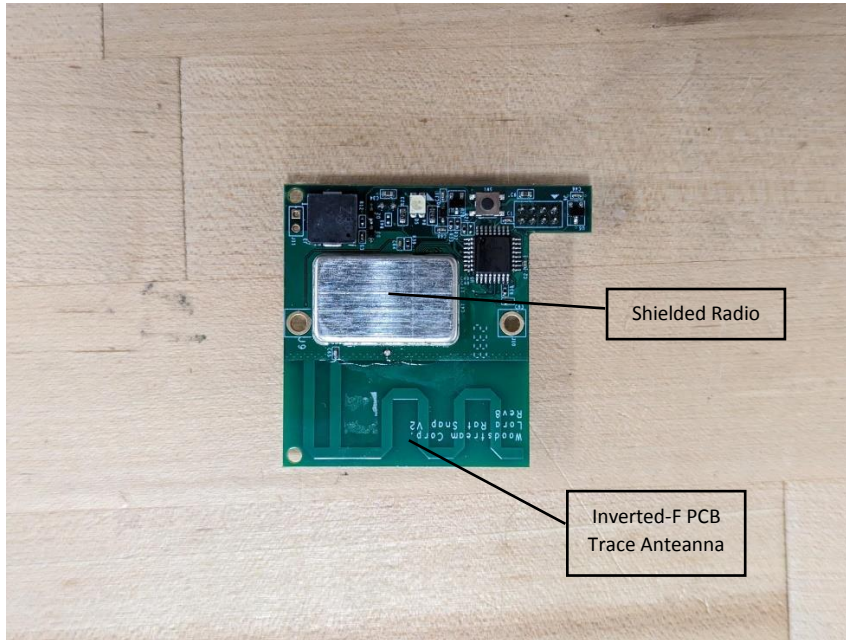
PCB Top Side with Radio Area Identified and with Shield
