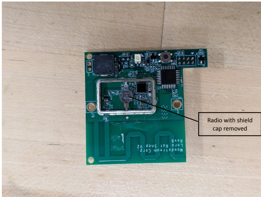
PCB Top Side with Radio with Shield Removed
