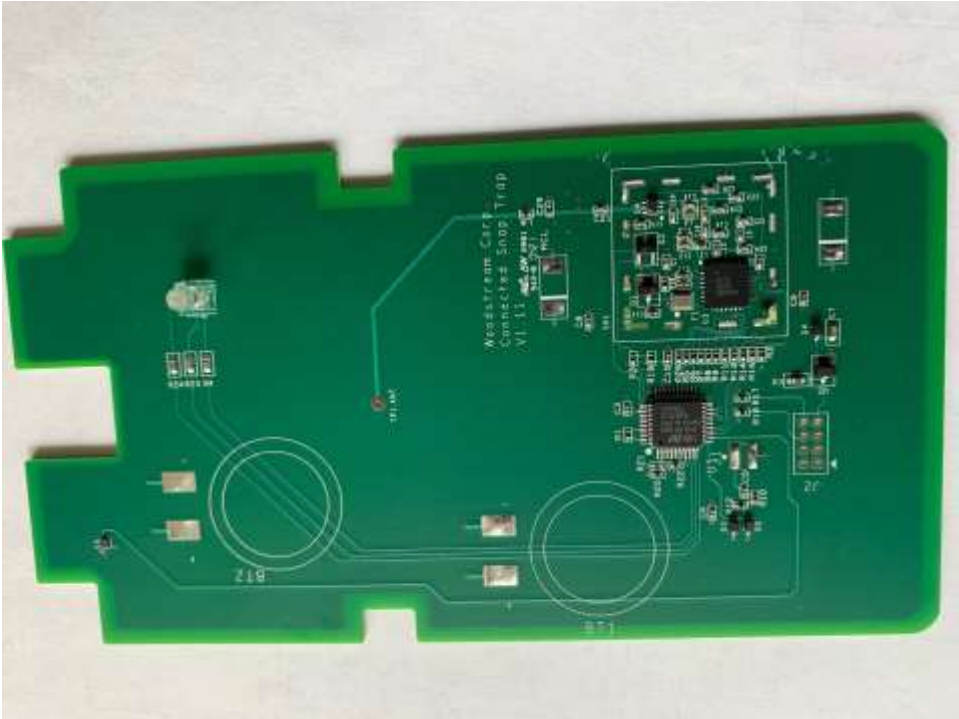
WOODSTREAM V430 TOP BOARD WITHOUT SHIELD
