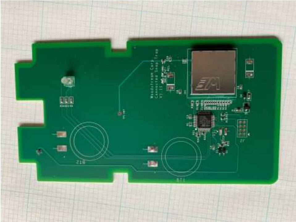
WOODSTREAM V430 TOP BOARD WITH SHIELD
