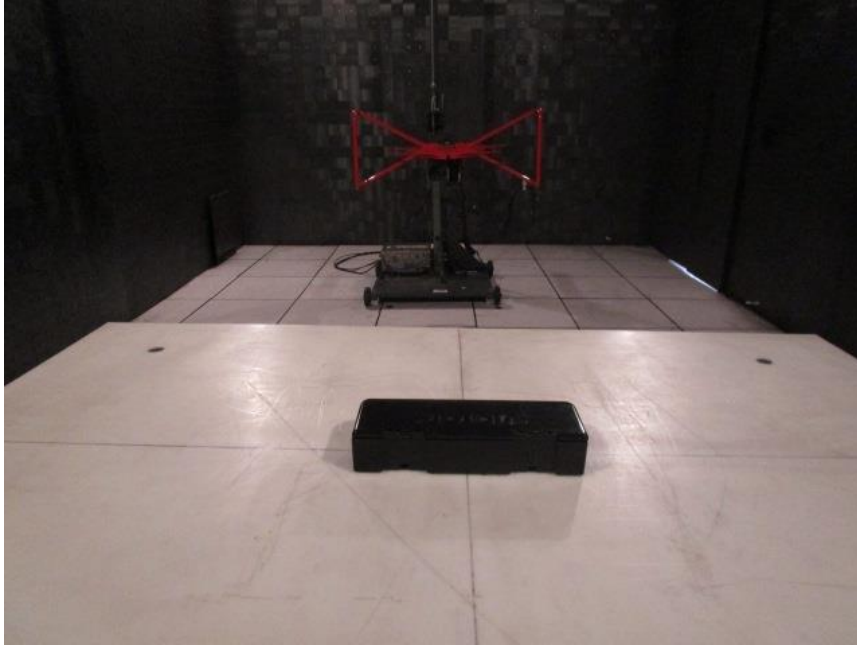
SHIELDED ROOM 3 METER 30-1000 MHZ
