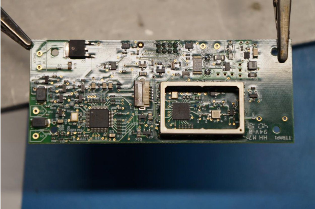
BOARD WITH SHIELD REMOVED
