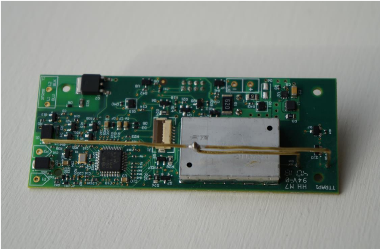
BOARD SIDE WITH SHIELD
