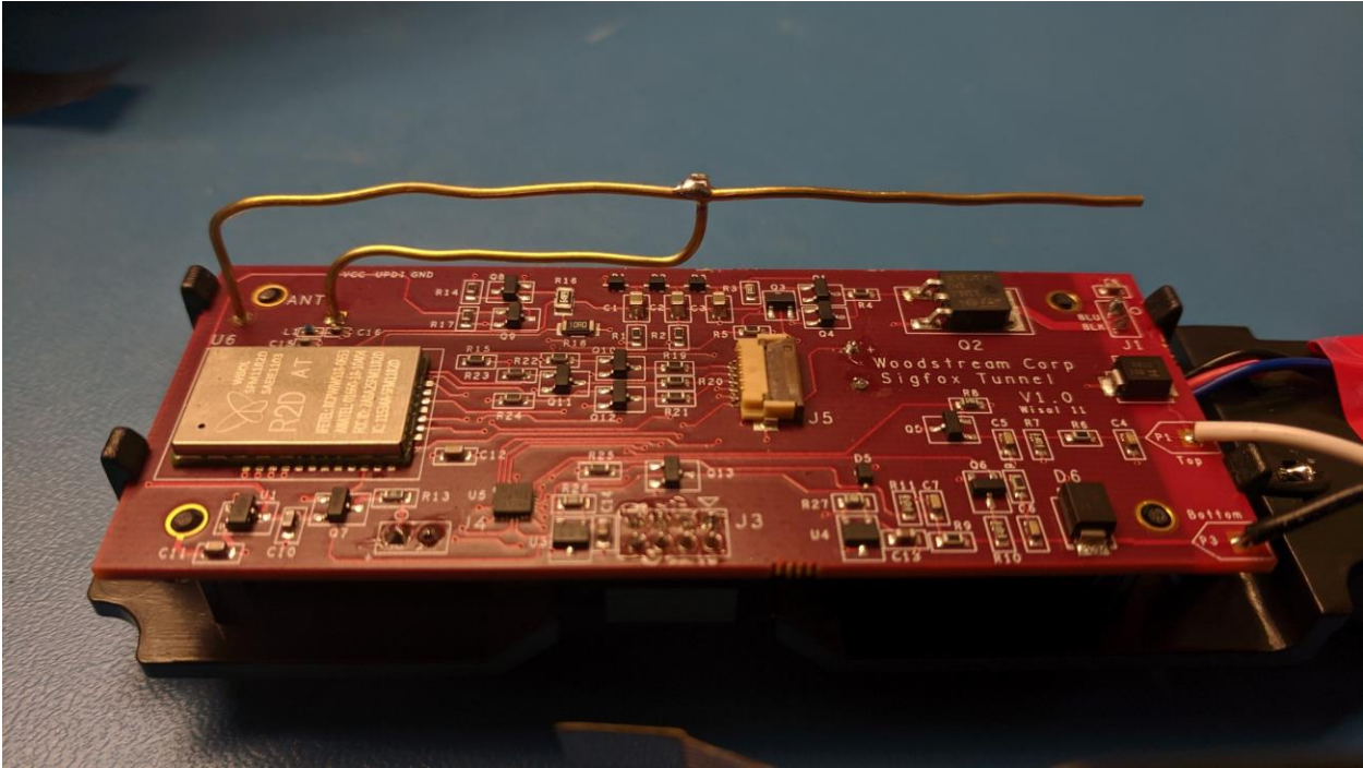
Woodstream V400S Antenna With WISOL SFM11R2D SigFox Module
