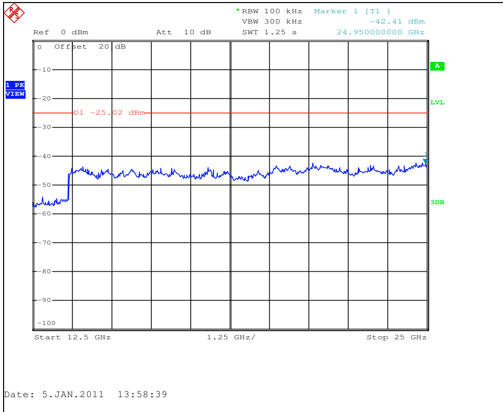
Figure 7.6.1.2-3: 12.5 GHz – 25 GHz
