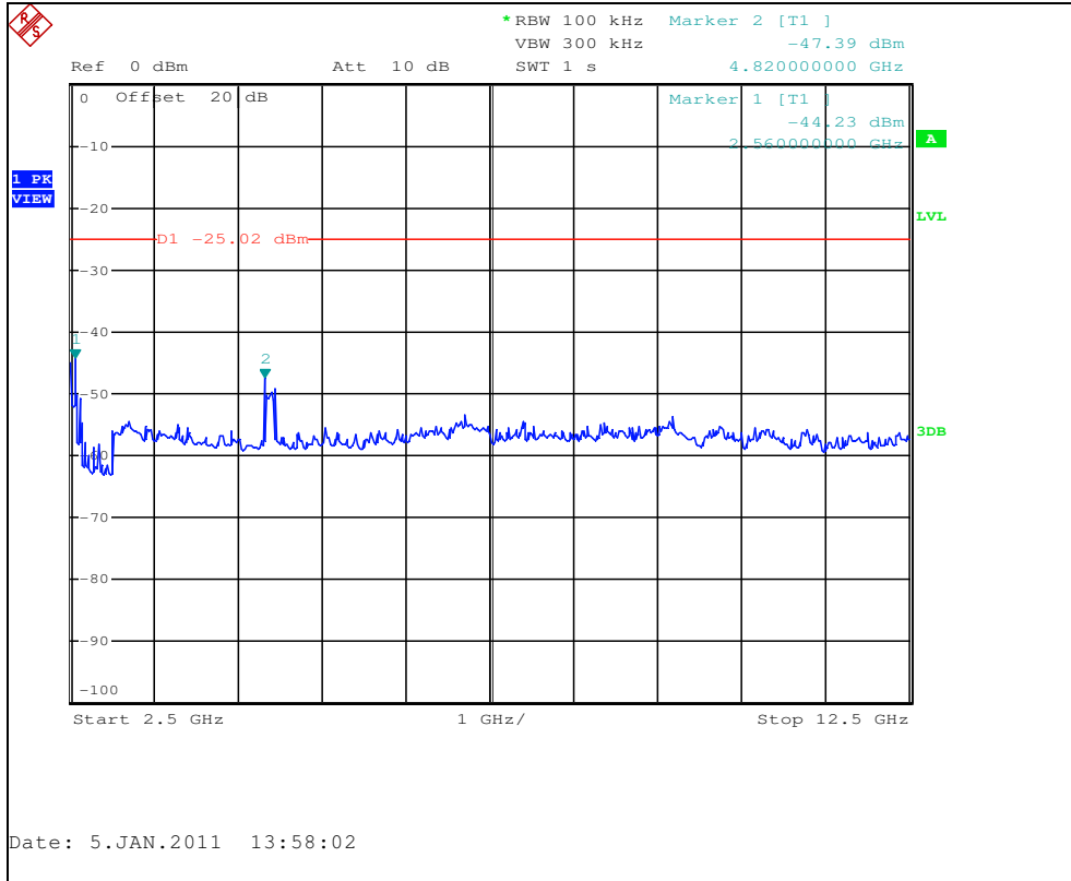
Figure 7.6.1.2-2: 2.5 GHz – 12.5 GHz
