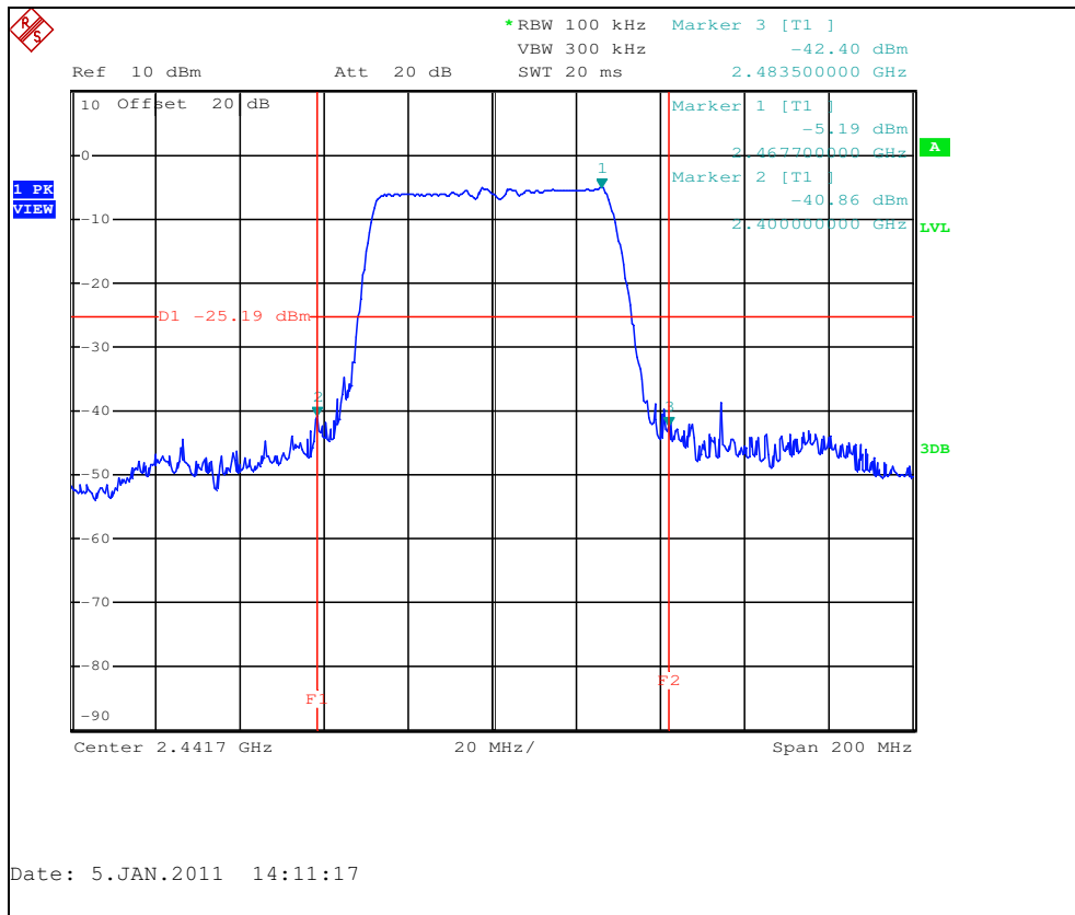
Figure 7.6.1.2-4: Band-edge (Conducted)
