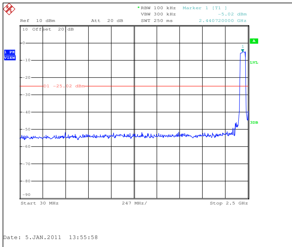
Figure 7.6.1.2-1: 30 MHz – 2.5 GHz
