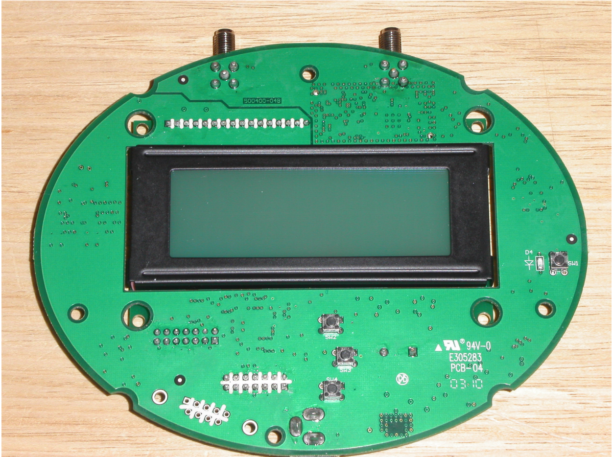
Figure 1: PCB - Front
