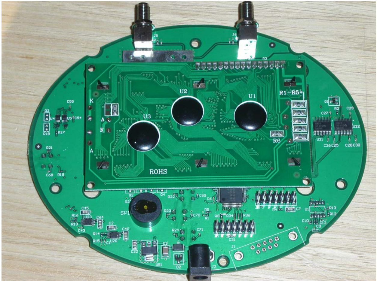
Figure 2: PCB - Back
