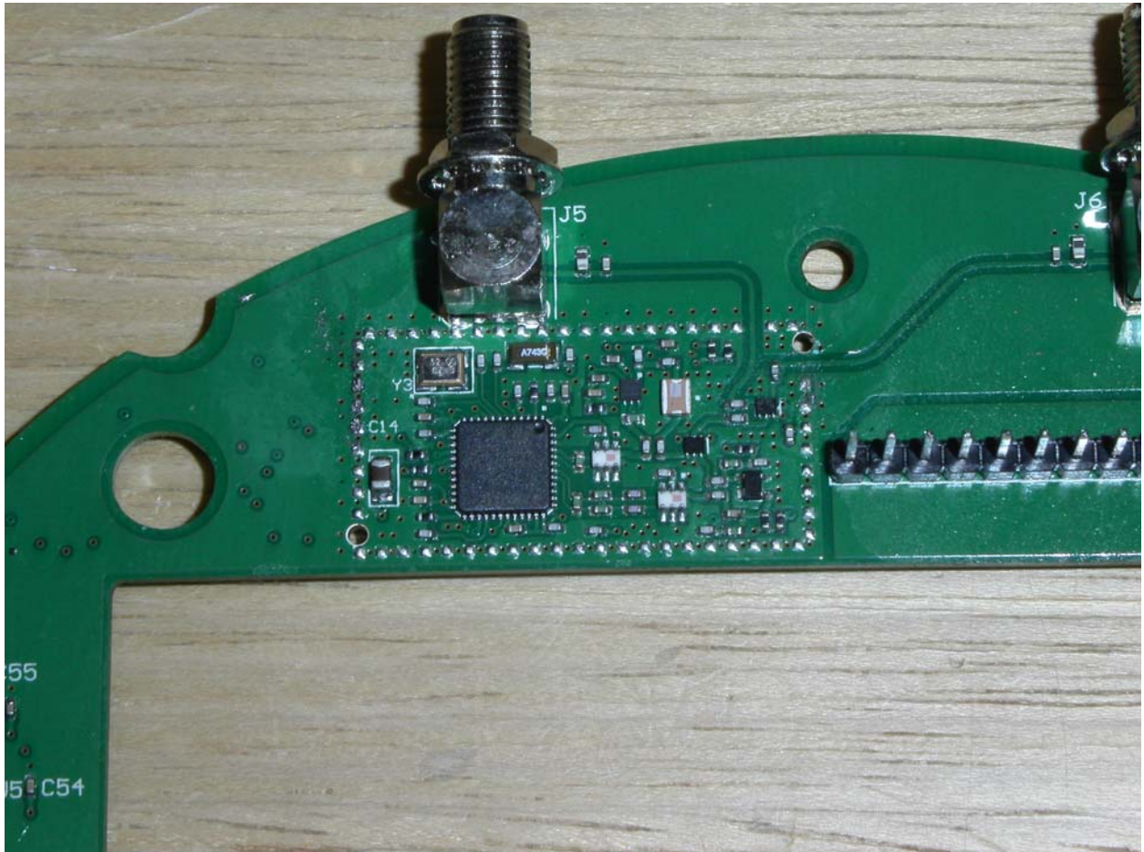
Figure 3: PCB without Shields - Back
