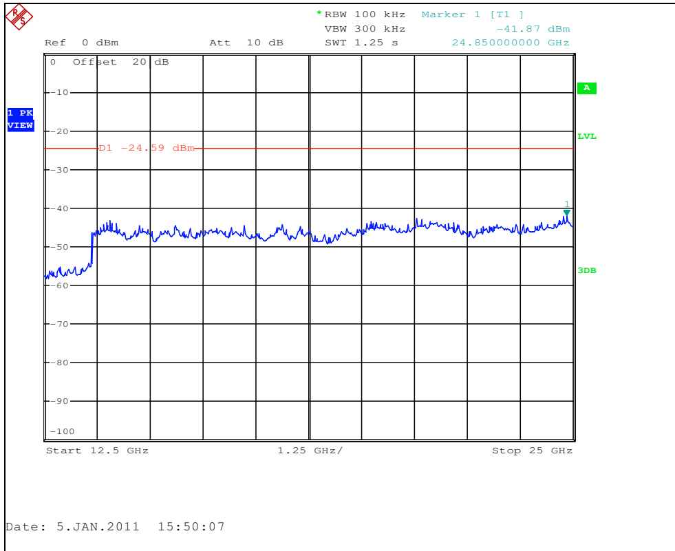
Figure 7.6.1.2-3: 12.5 GHz – 25 GHz
