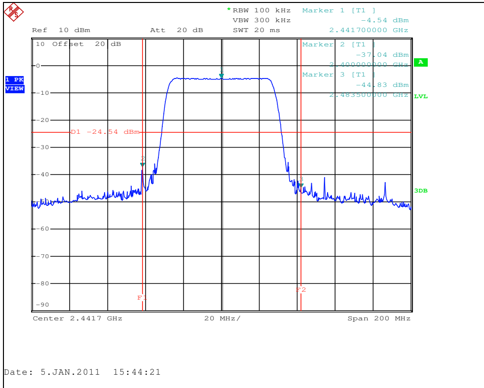
Figure 7.6.1.2-4: Band-edge (Conducted)
