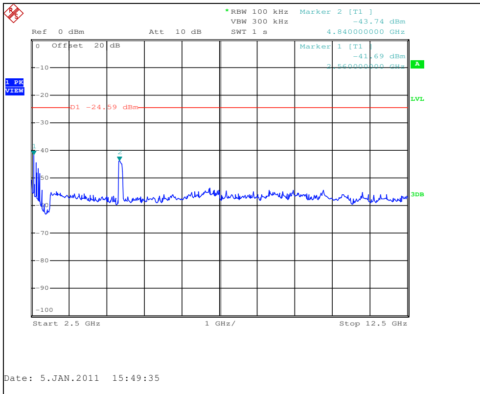
Figure 7.6.1.2-2: 2.5 GHz – 12.5 GHz
