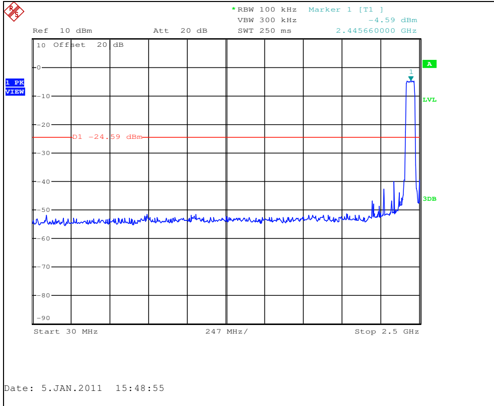
Figure 7.6.1.2-1: 30 MHz – 2.5 GHz
