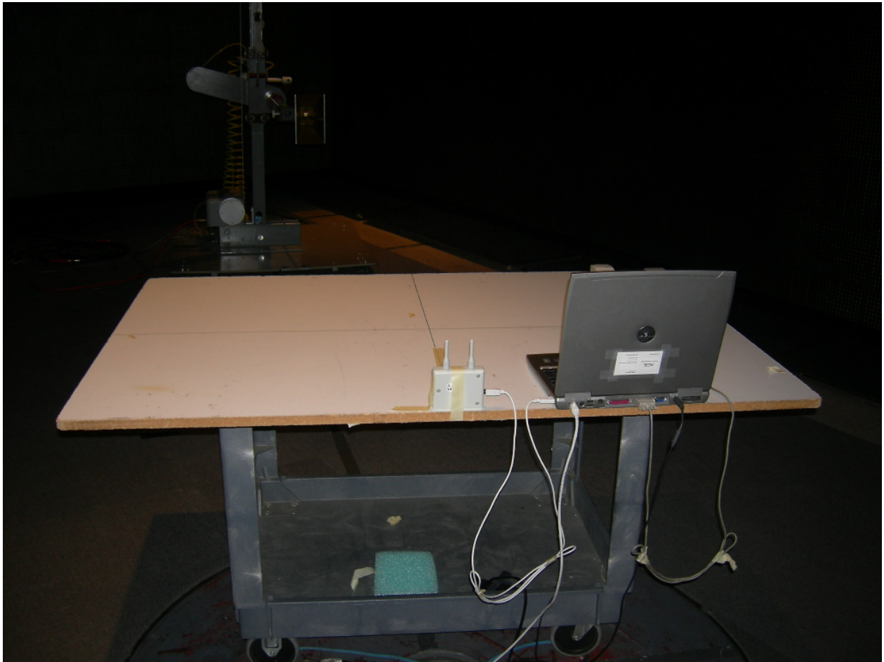
Figure 3: Radiated Emissions
