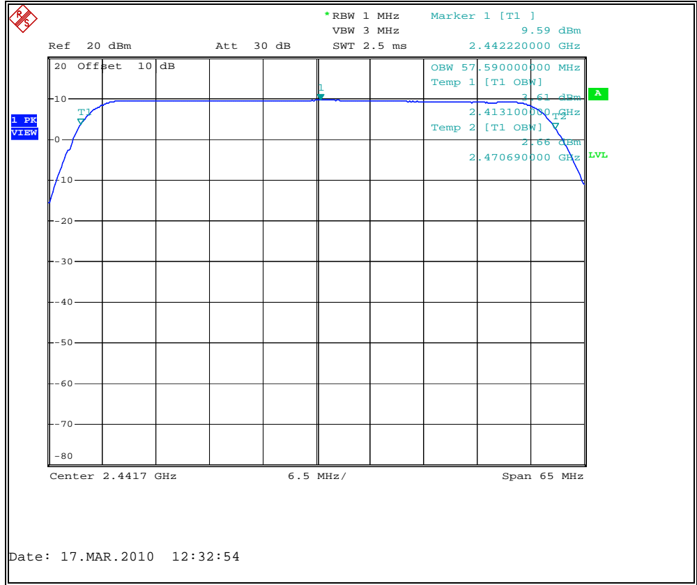
Figure 7.4.2-2: 99% Bandwidth Plot
