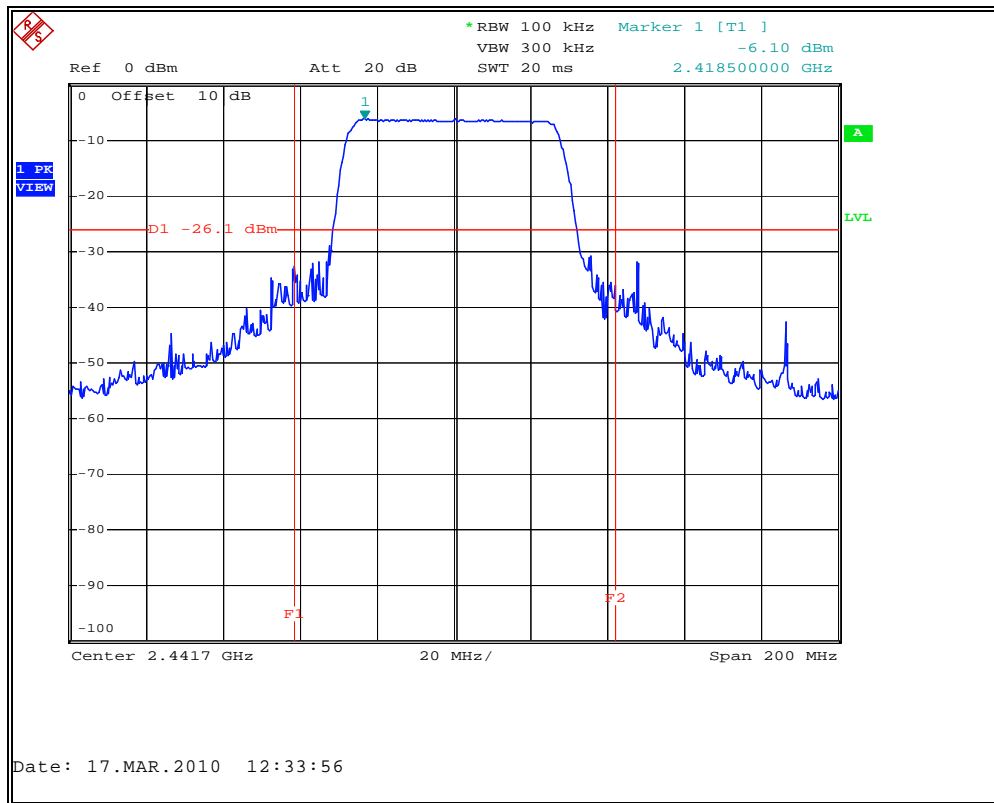
Figure 7.6.2.2-4: Band-edge (Conducted)
