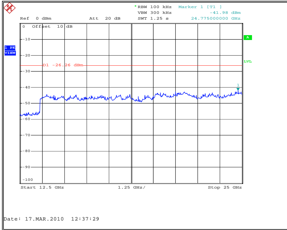
Figure 7.6.2.2-3: 12.5 GHz – 25 GHz
