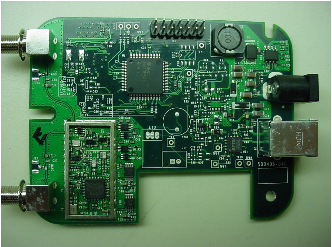
Figure 2: PCB without Shields - Front
