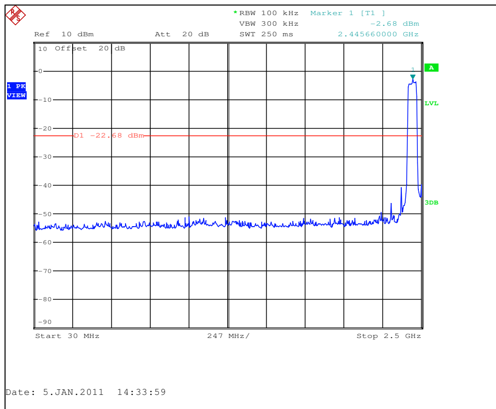
Figure 7.6.1.2-1: 30 MHz – 2.5 GHz
