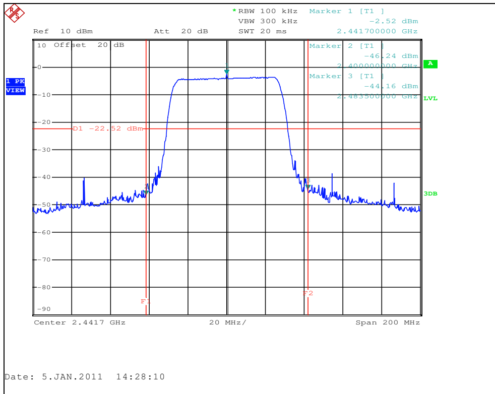
Figure 7.6.1.2-4: Band-edge (Conducted)
