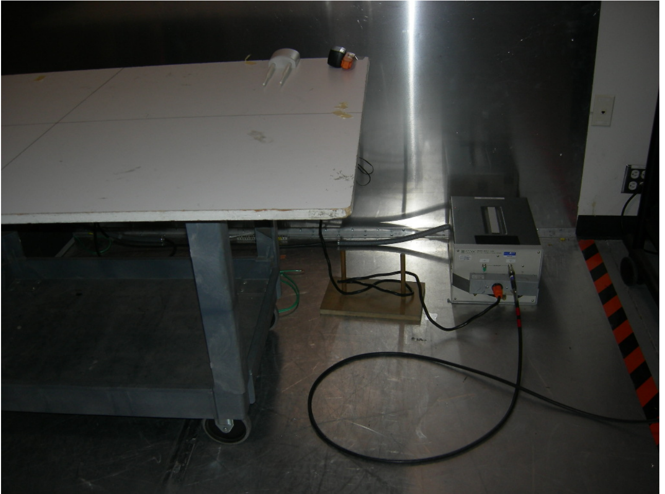
Figure 4: AC Power Line Conducted Emissions
