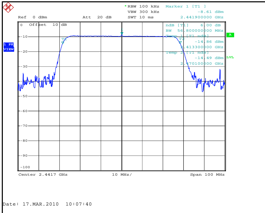
Figure 7.4.2-1: 6dB Bandwidth Plot
