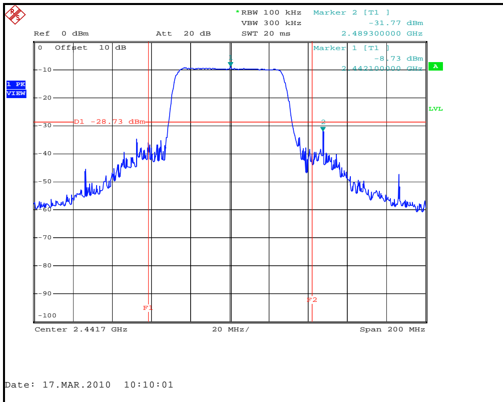
Figure 7.6.2.2-4: Band-edge (Conducted)
