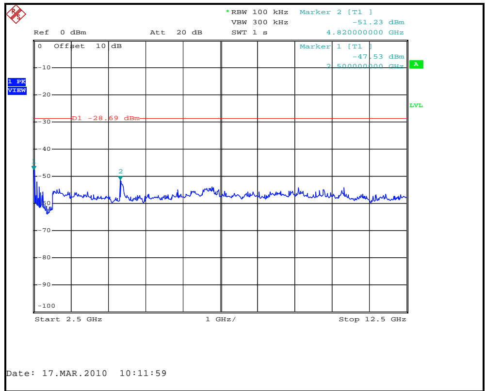
Figure 7.6.2.2-2: 2.5 GHz – 12.5 GHz
