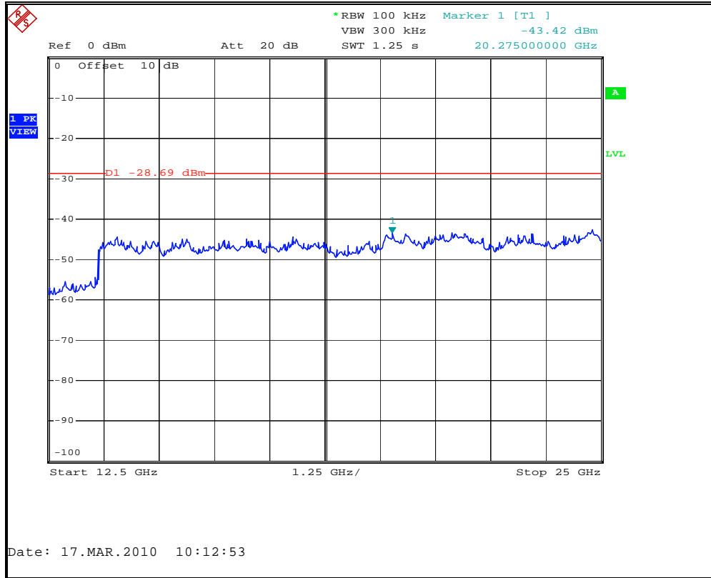
Figure 7.6.2.2-3: 12.5 GHz – 25 GHz
