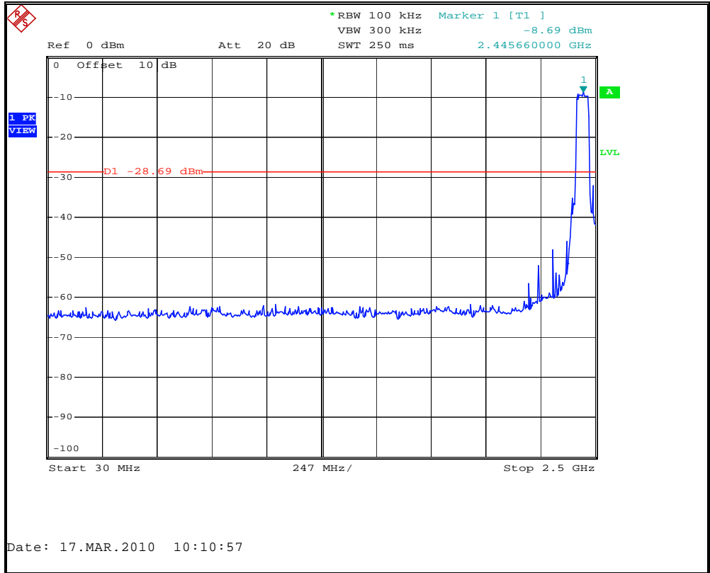
Figure 7.6.2.2-1: 30 MHz – 2.5 GHz
