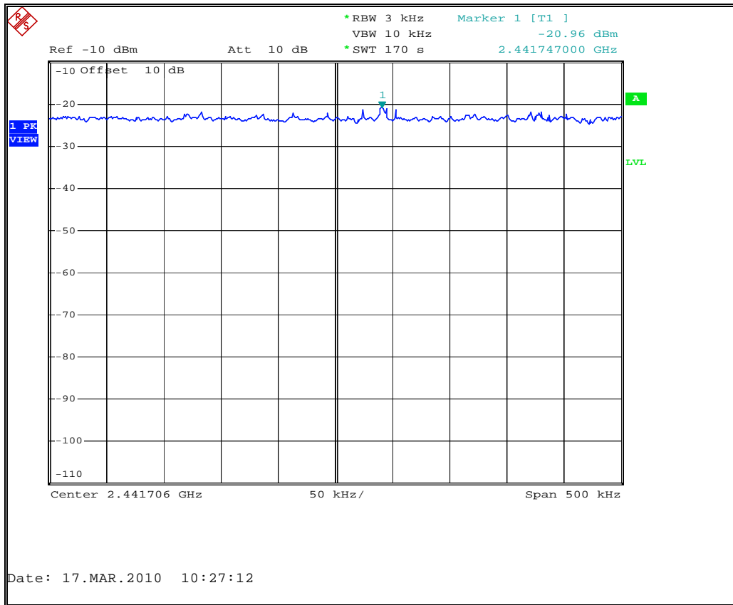
Figure 7.7.2-1: Power Spectral Density Plot
