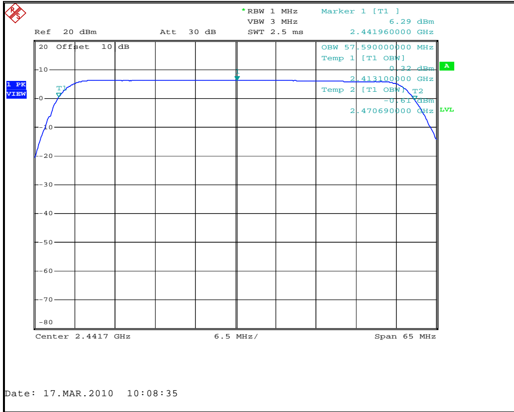
Figure 7.4.2-2: 99% Bandwidth Plot
