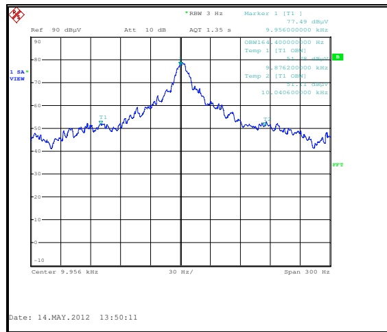
Figure 7.4.2-2: 99% Bandwidth Plot
