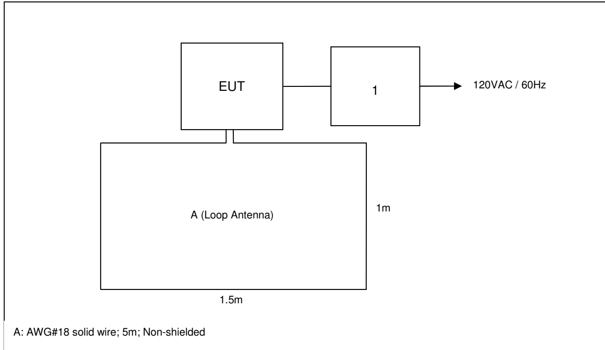
Figure 6-1: Test Setup Block Diagram
